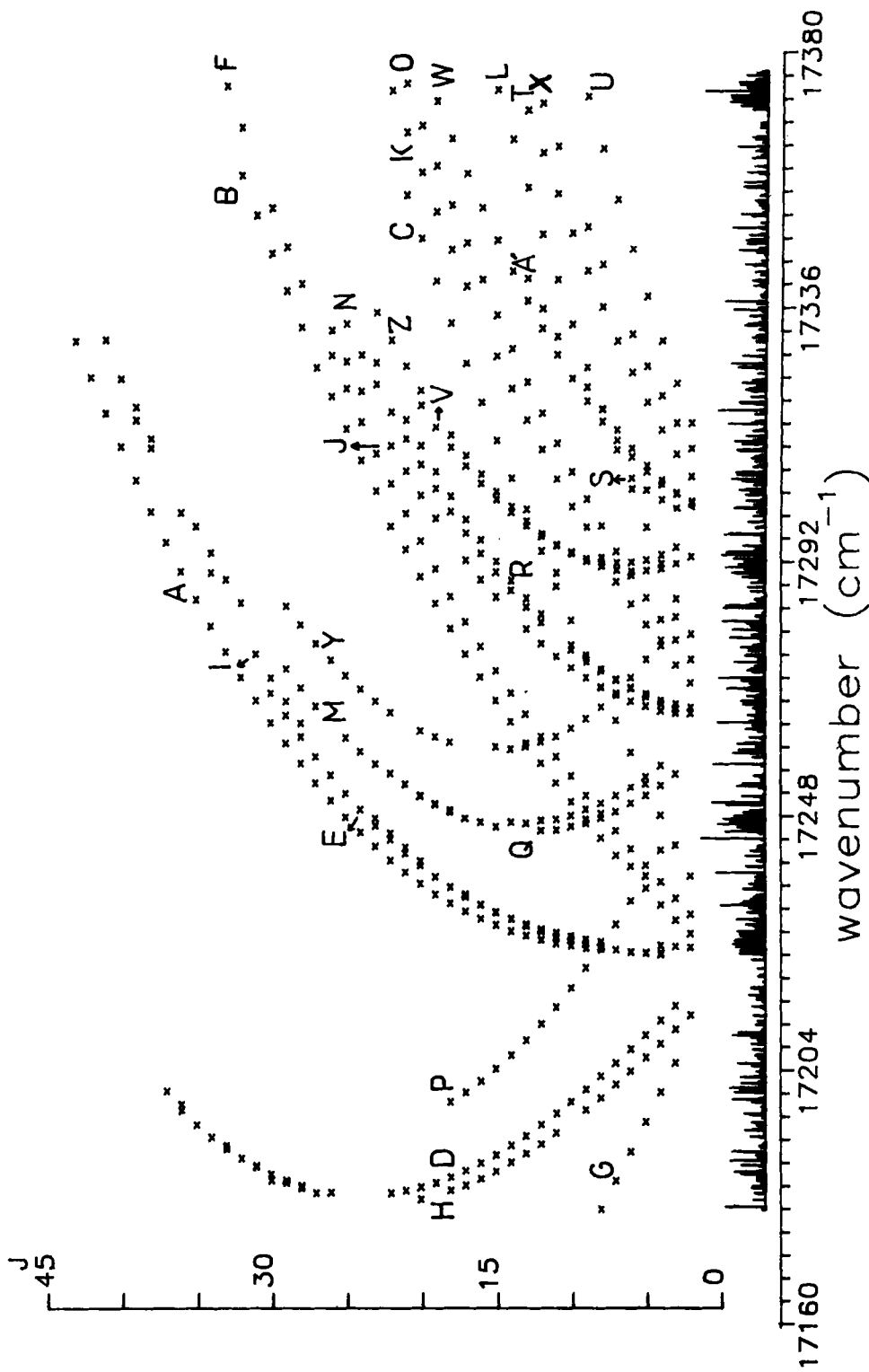
Figure 2. Optogalvanic spectrum along with Fortrat diagram of the (11, 7) band in the B^3\Pi_g - A^3\Sigma_u^+ transition of N_2 from 17179 to 17376\text{ cm}^{-1} . (27 branches namely P_{11}, Q_{11}, \dots, Q_{33} and R_{33} are indicated as by A, B, ..., Z and A' respectively.)
