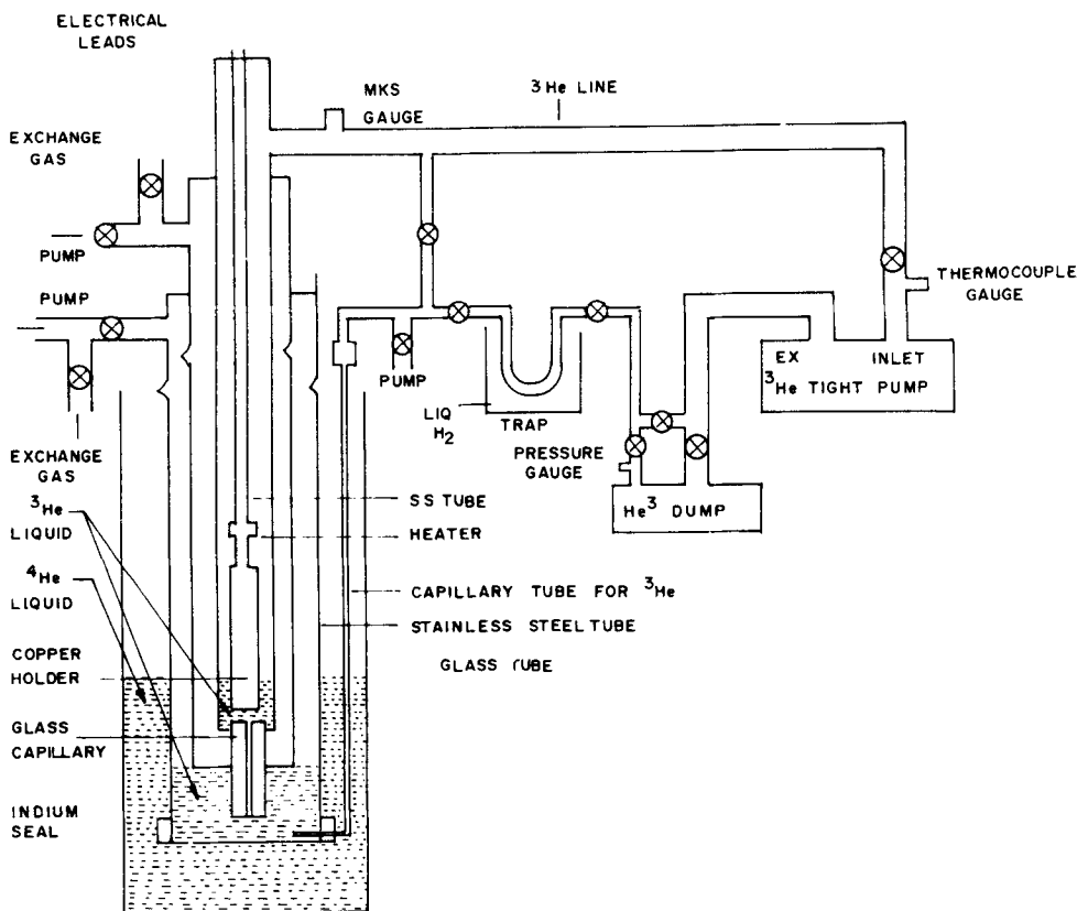
Figure 2. The ^3\text{He} gas handling assembly.
