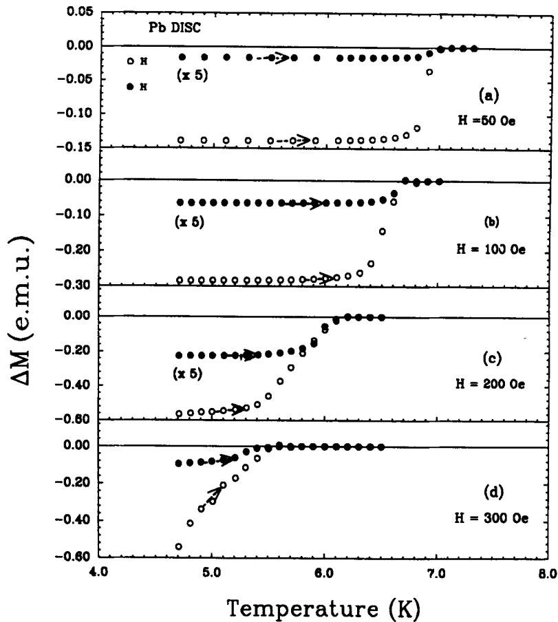
Figure 3. Plots of \Delta M(H)(= (M_{FC}(H) - M_{ZFC}(H))) vs T in Pb disc for field applied parallel (open circle) and perpendicular (close circle) to the disc plane. The arrows mark the T_r(H) values by \Delta M(H) \rightarrow 0 criterion.
