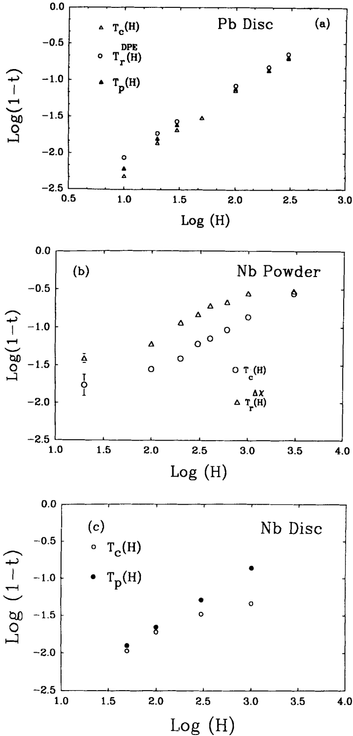
Figure 11. Log-log plots of (1-t) vs H for different sets of t values in Pb disc (a), Nb powder (b) and Nb disc (c) specimens. The three sets of t values in Pb correspond to T_c(H)/T_c(0) , T_r^{\text{DPE}}(H)/T_c(0) (DPE at 21 Hz) and T_p(H)/T_c(0) respectively. The two sets each in Nb powder and disc specimens correspond to T_c(H)/T_c(0) and T_r^{\Delta x}(H)/T_c(0) , and T_c(H)/T_c(0) and T_p(H)/T_c(0) respectively.
