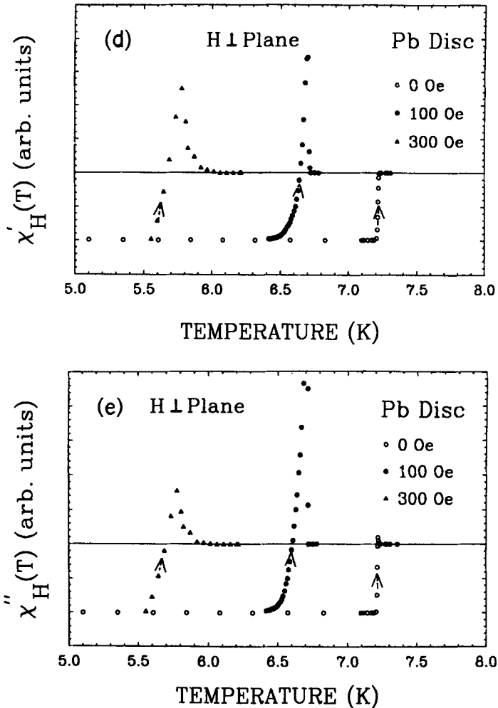
Figure 4. The temperature variation of \chi'_H and \chi''_H (measured at 21 Hz in h_{ac} of 1 Oe rms) in Pb disc specimen in the parallel ((a), (b) and (c)) and perpendicular ((d) and (e)) orientations. The data at different H values have not been scaled to one-another. Wherever considered appropriate, the horizontal lines have been drawn through susceptibility values in the normal state for reference purpose only.
