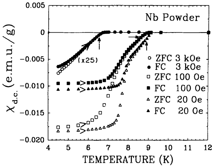
Figure 8. The temperature variation of ZFC and FC DC susceptibility values in Nb powder specimen at H = 20, 100, 3000 Oe respectively. The arrows identify the T_c(H) values by \Delta\chi(H) \rightarrow 0 criterion.
