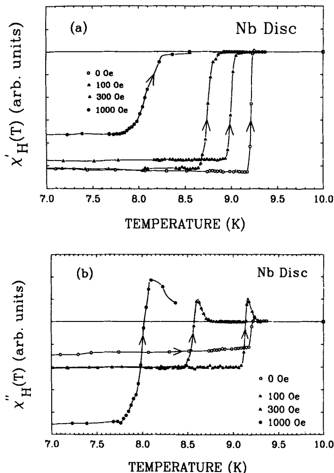
Figure 10. The temperature variation of \chi'_H and \chi''_H measured at 21 Hz in h_{ac} of 1 Oe in Nb disc at field values indicated in the parallel orientation. The continuous line joining the data points are just an aid to guide the eye. The data sets at different H are not normalized to one-another.
