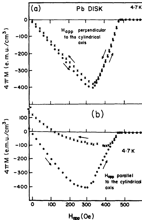
Figure 1. Magnetization hysteresis curve in Pb disc (dia = 4.15 mm, thickness = 2.15 mm) at 4.7 K for field applied nominally parallel and perpendicular to the disc plane.
