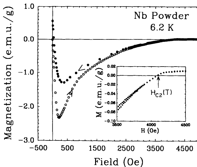
Figure 7. Magnetization hysteresis curve in Nb powder specimen at 6.2 K. The inset shows the forward and reverse M - H curves near H_{c2} value.
