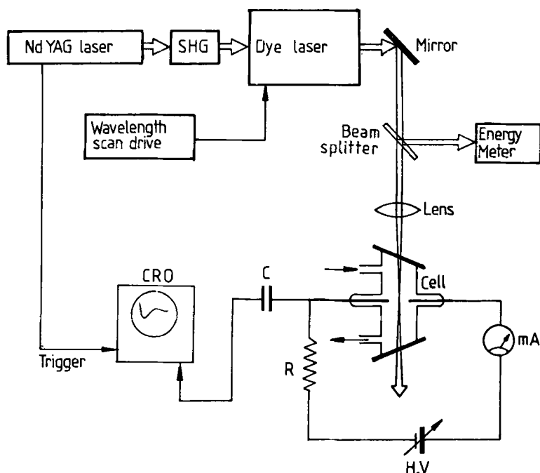
Figure 1(a). Schematic diagram of the experimental set up.
