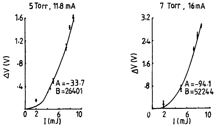
Figure 3. Curve for \Delta V = AI + BI^2 at 5 torr and 7 torr, I is the laser energy per pulse. Points correspond to experimental observations.
