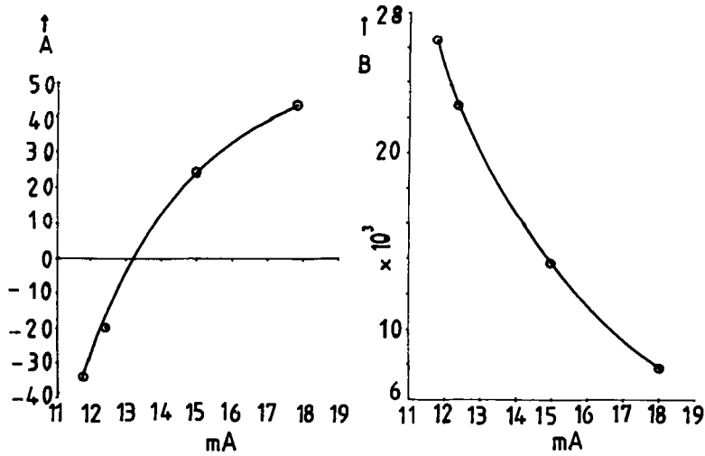
Figure 4(a). Variation of coefficients A [in V/J] and B [in V/J 2 ] with discharge current at 5 torr.
