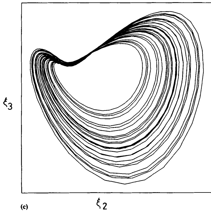
Figure 3a-c. Corresponding portraits obtained by solving the model equations given by table 1. These figures are to be compared with figure 2.
