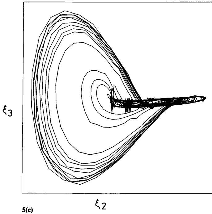
Figure 5. Phase space portraits of the attractor reconstructed from x time series of the Rossler system. Figures (a), (b) and (c) show \xi_1 \xi_2 , \xi_1 \xi_3 and \xi_2 \xi_3 projections of the attractor respectively.
