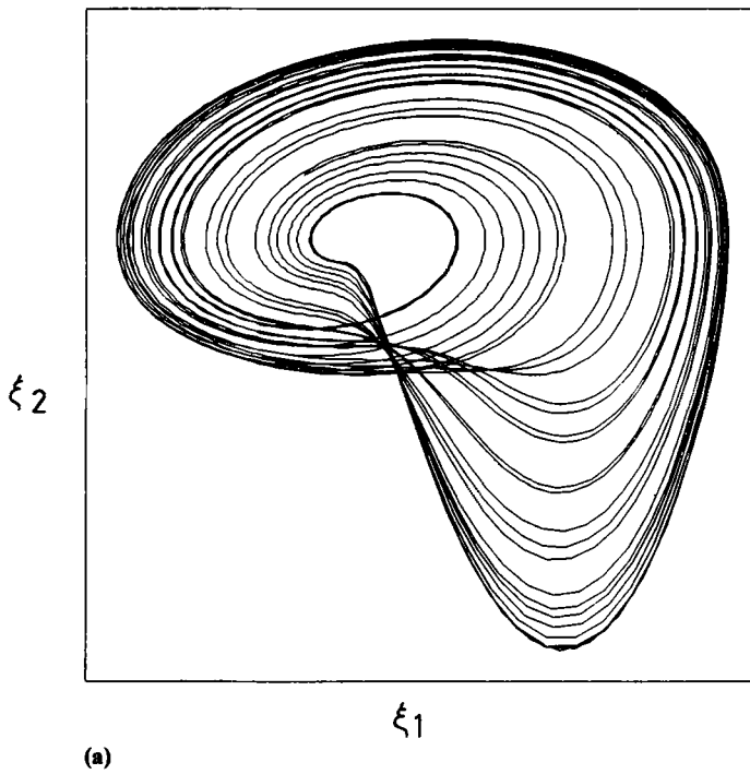
Figure 5. Phase space portraits of the attractor reconstructed from x time series of the Rossler system. Figures (a), (b) and (c) show \xi_1 \xi_2 , \xi_1 \xi_3 and \xi_2 \xi_3 projections of the attractor respectively.
