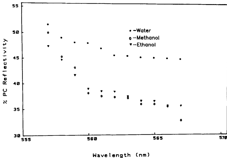
Figure 6. Percentage reflectivities as a function of wavelength for RhB in different solvents.
