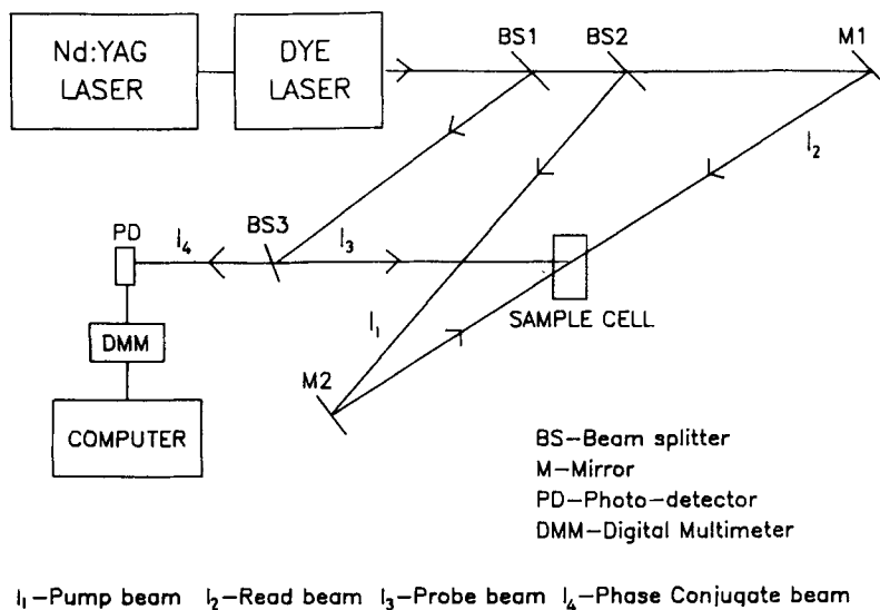
Figure 2. Experimental arrangement for studying dependence of phase conjugate reflectivity on absorption spectrum by DFWM.
