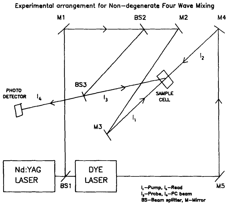
Figure 7. Experimental arrangement to study the thermal grating characteristics using NFWM.
