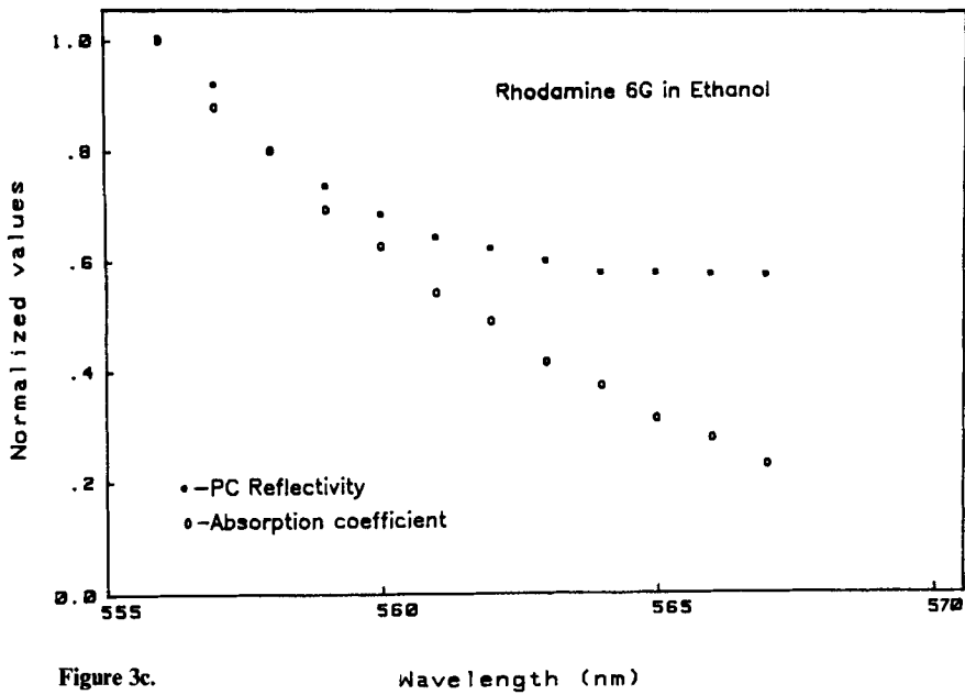
Figure 3a-c. Variation of absorption coefficient and phase conjugate reflectivity with wavelength for Rh6G in water, methanol and ethanol.
