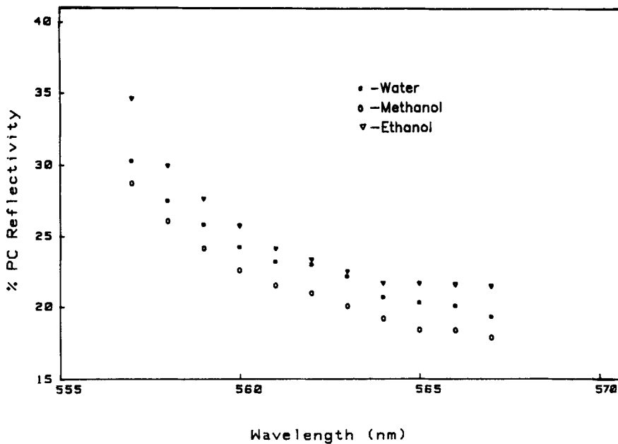
Figure 5. Percentage reflectivities as a function of wavelength for Rh6G in different solvents.
