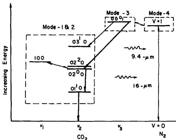
Figure 1b. Schematic diagram of vibrational energy levels of \text{CO}_2 and \text{N}_2 molecules.
