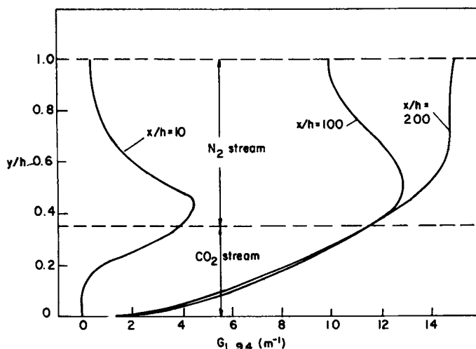
Figure 9. Transverse profiles of local small-signal gain at various axial locations in the cavity.
