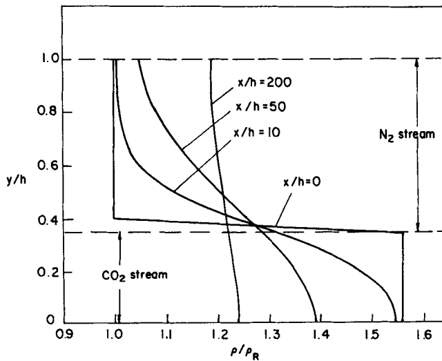
Figure 3. Transverse mixture-density distribution profiles at various axial locations in the cavity.
