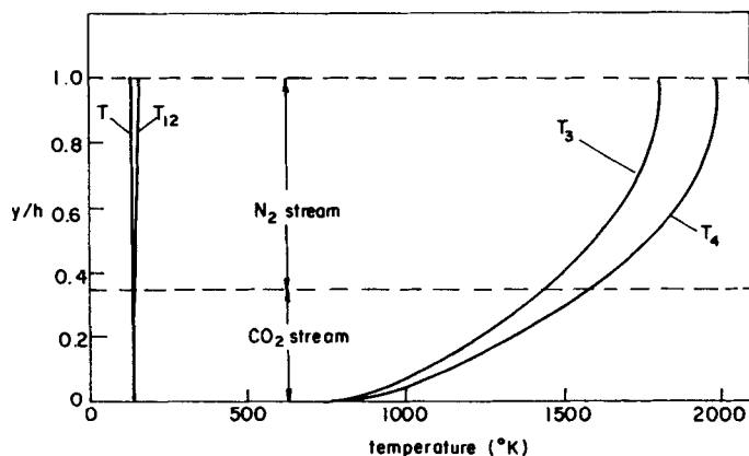
Figure 8. Transverse profiles of static temperature ( T ) and vibrational temperatures of the modes (12), (3) and (4) at x/h = 200 .
