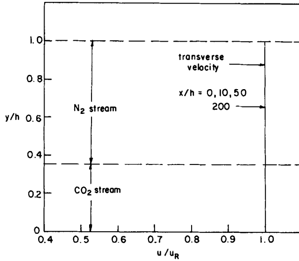
Figure 2. Transverse velocity distribution profiles at various axial locations in the cavity.
