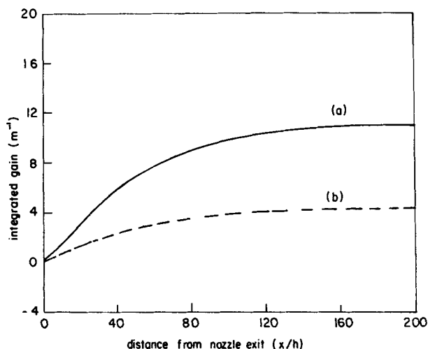
Figure 10. Variation of average small-signal gain (integrated gain) along the flow for (a) Lorentzian broadening and (b) Lorentzian-Doppler broadening.
