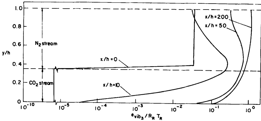
Figure 5. Transverse profiles of vibrational energy in mode-3 at various axial locations in the cavity.
