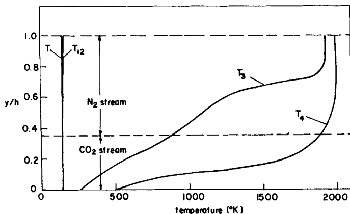
Figure 7. Transverse profiles of static temperature ( T ) and vibrational temperatures of the modes (12), (3) and (4) at x/h = 10 .
