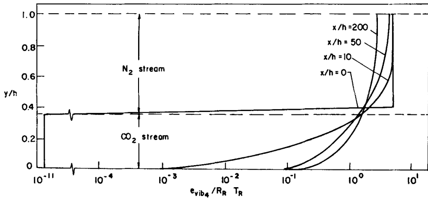
Figure 4. Transverse profiles of vibrational energy in mode-4 at various axial locations in the cavity.
