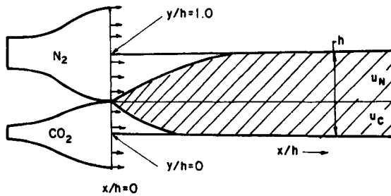
Figure 1a. Schematic diagram of a downstream-mixing gasdynamic laser.
