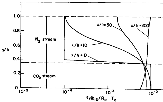
Figure 6. Transverse profiles of vibrational energy in mode-12 at various axial locations in the cavity.
