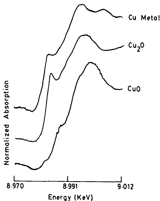
Figure 1. Normalized Cu K-edge XANES of Cu metal, \text{Cu}_2\text{O} and \text{CuO} .
