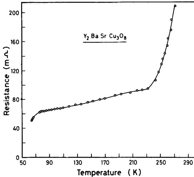
Figure 1. Resistive transition curve for the sample Y_2BaSrCu_3O_8 .
