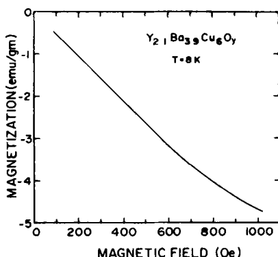
Figure 7. Magnetization as a function of the applied magnetic field at 8 K for the oxygen-presintered specimen of the Y_{2.1}Ba_{3.9}Cu_6O_y .
