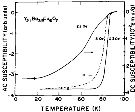
Figure 4. AC susceptibility (in two measuring fields 0.3 Oe and 3 Oe) and DC susceptibility (in a field of 22 Oe) as a function of temperature for the oxygen-presintered specimen of Y_{2.1}Ba_{3.9}Cu_6O_y .
