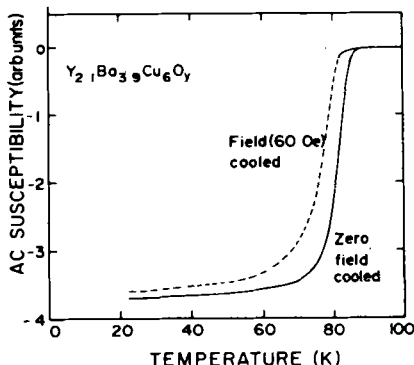
Figure 5. AC susceptibility of the oxygen-presintered specimen of the composition Y_{2.1}Ba_{3.9}Cu_6O_y in the presence of DC field (60 Oe) as well as in the absence of this field.
