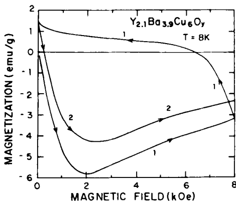
Figure 6. Magnetic hysteresis curve (measured up to a field of 8 kOe) for the oxygen-presintered specimen of Y_{2.1}Ba_{3.9}Cu_6O_y .
