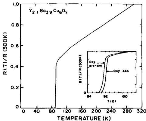
Figure 3. Resistance (4.2–300 K) normalized to the 300 K value for the oxygen presintered specimen of the sample Y_{2.1}Ba_{3.9}Cu_6O_y . Inset shows the difference in the resistance data for the oxygen-presintered and oxygen-annealed specimens of the same composition.
