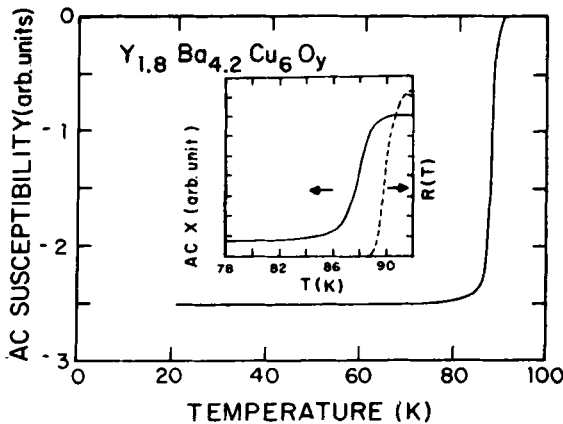
Figure 2. AC susceptibility ( \chi ) in the temperature interval 20–100 K for the specimen Y_{1.8}Ba_{4.2}Cu_6O_y . Inset shows AC \chi as well as the resistance data in the temperature interval 78–92 K for the same specimen.
