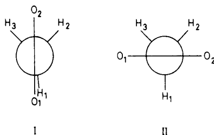
Figure 1. Two conformers of nitromethane.
