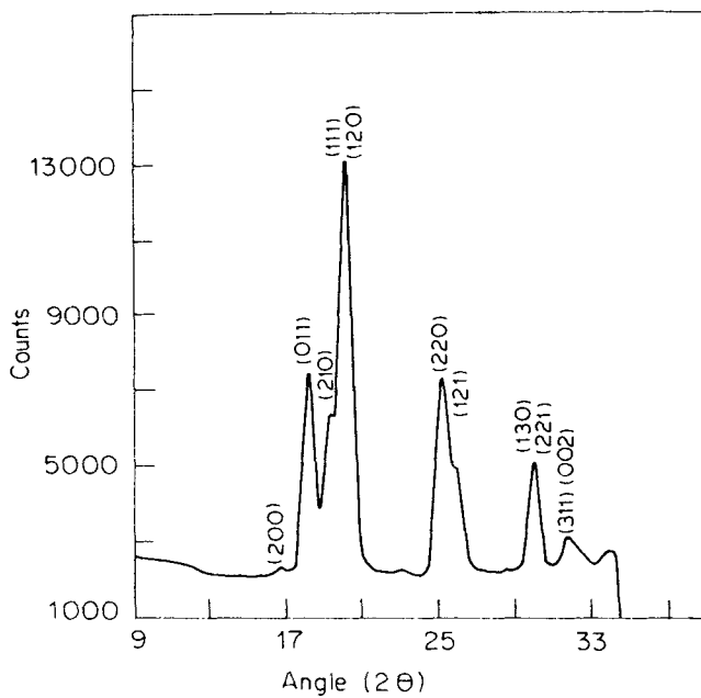
Figure 1. The diffraction pattern of \alpha -resorcinol at ambient conditions ( \lambda = 1.5418 \text{ \AA} ).
