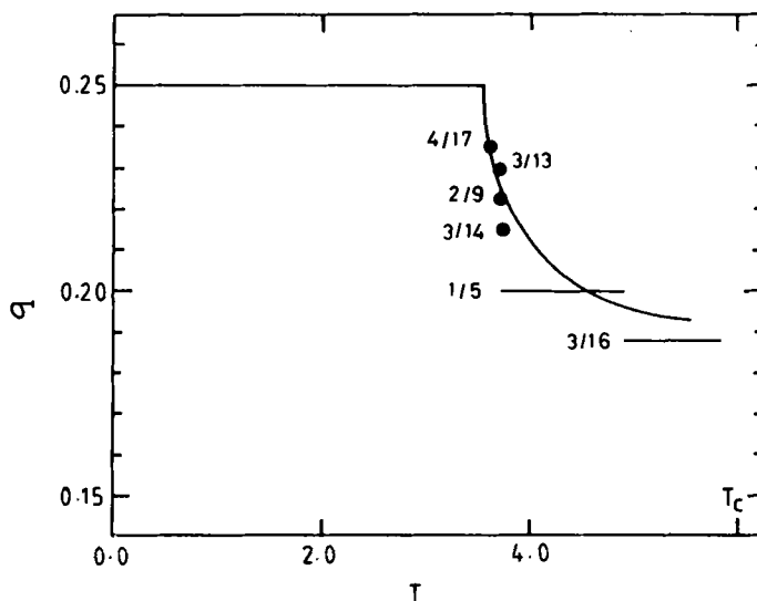
Figure 1. Equilibrium wavevector vs temperature for J_2/J_1 = -0.7 . The dots and the horizontal lines are results of numerical mean field calculations. Full curve is the result of soliton theory (Bak and von Boehm 1980).
