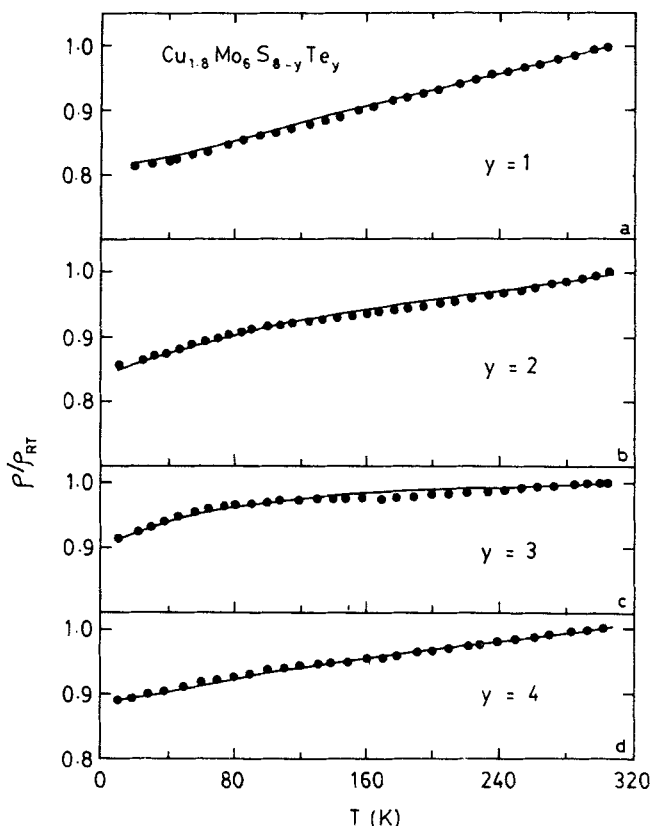
Figure 1. Variation of normalised electrical resistivity of \text{Cu}_{1.8}\text{Mo}_6\text{S}_{8-y}\text{Te}_y , 1 \leq y \leq 4 as a function of temperature, points-experimental, continuous curve-fitted to Cote-Meisel theory.
