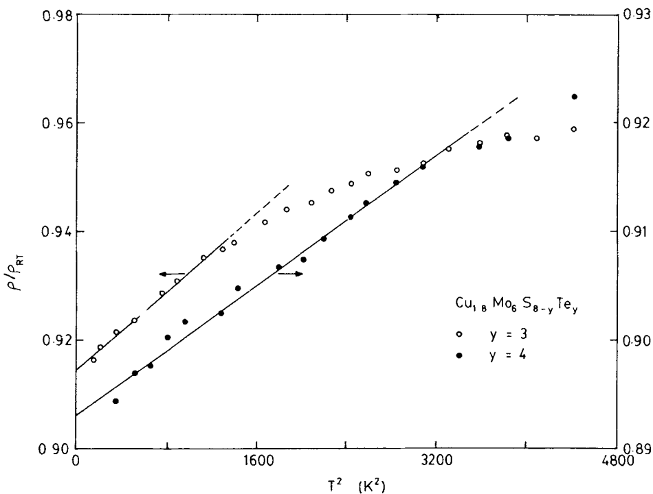
Figure 3. Variation of normalised electrical resistivity of \text{Cu}_{1.8}\text{Mo}_6\text{S}_{8-y}\text{Te}_y as a function of square of the temperature for y = 3 and 4.
