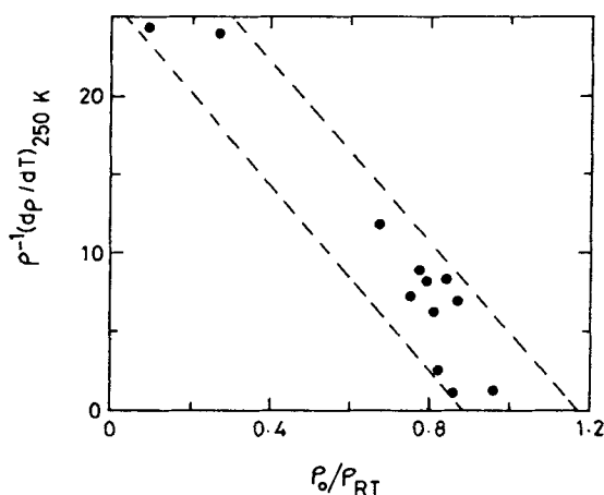
Figure 4. Plot of \rho^{-1} (d\rho/dT) at 250 K as a function of residual resistivity ratio \rho_0/\rho_{RT} .
