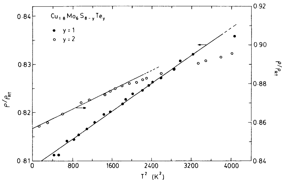
Figure 2. Variation of normalised electrical resistivity of \text{Cu}_{1.8}\text{Mo}_6\text{S}_{8-y}\text{Te}_y as a function of square of the temperature for y = 1 and 2.
