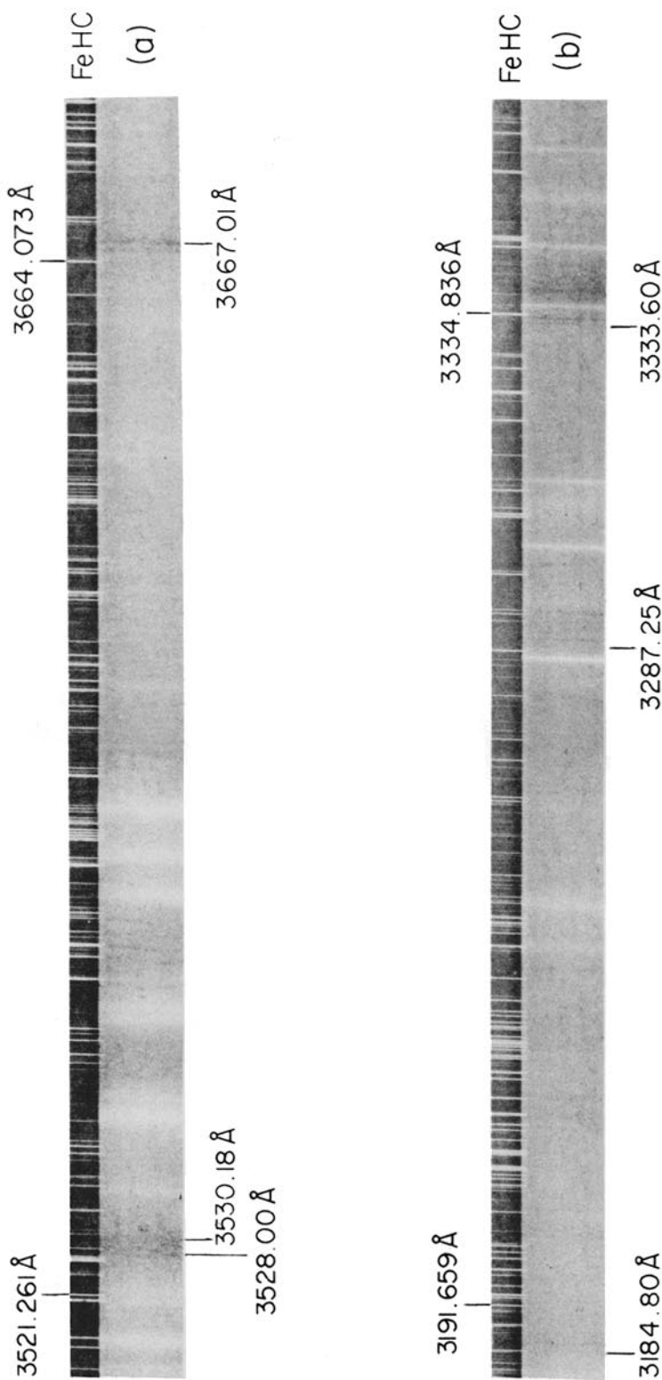
Figure 1. Absorption bands of HCCO radical obtained in the flash photolysis of isoxazole-argon mixture. a. 3400–3670 Å system. b. 3080–3400 Å system.
