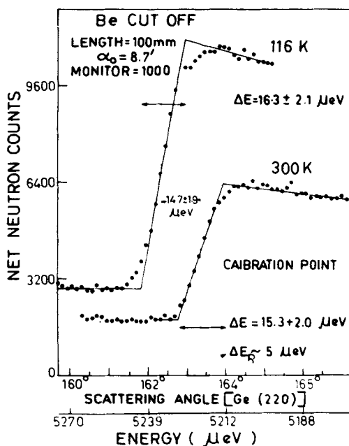
Figure 3. Energy analysis of beam transmitted through 100 mm Be at 300 K and 116 K.
