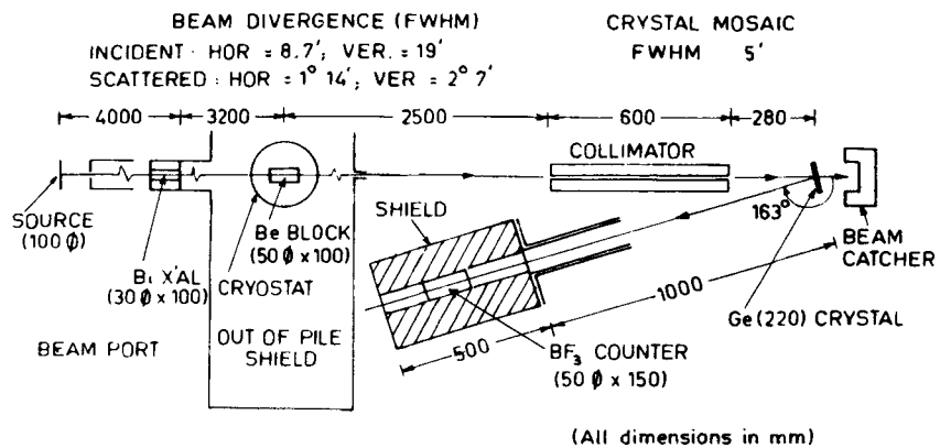
Figure 1. Schematic layout of the single crystal spectrometer used for high resolution Bragg cut-off measurements.
