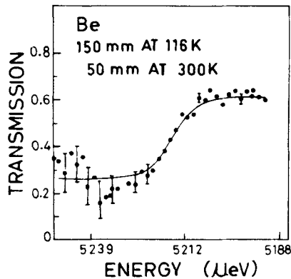
Figure 4. Transmission of 50 mm Be at 300 K as a function of energy as measured with beam transmitted through cooled Be (150 mm long at 116 K).
