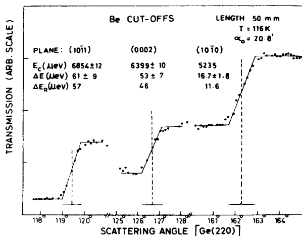
Figure 5. Energy analysis of beam transmitted through 50 mm Be at 116 K for the Bragg planes (1010), (0002) and (1011).
