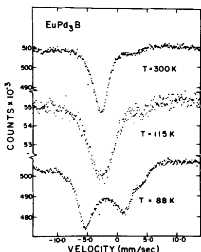
Figure 10. ^{151}\text{Eu} Mössbauer of \text{EuPd}_3\text{B} at various temperatures.
