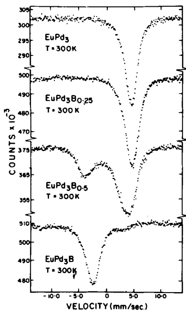
Figure 8. ^{151}\text{Eu} Mössbauer spectra in \text{EuPd}_3\text{B}_x ( x = 0, 0.25, 0.5 and 1.0 ) alloys at 300 K.
