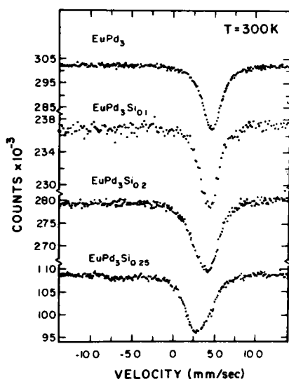
Figure 13. ^{151}\text{Eu} Mössbauer spectra of \text{EuPd}_3\text{Si}_x ( x = 0, 0.1, 0.2 and 0.25 ) alloys at 300 K.
