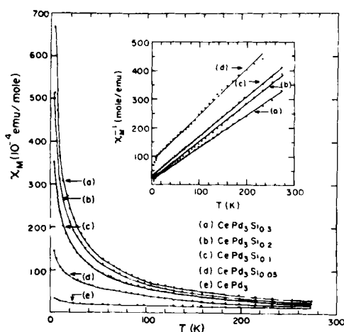
Figure 5. Susceptibility vs. temperature of \text{CePd}_3\text{Si}_x ( x = 0, 0.05, 0.1, 0.2 and 0.3 ) alloys.
