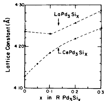
Figure 4. Lattice parameter of \text{LaPd}_3\text{Si}_x and \text{CePd}_3\text{Si}_x ( 0 \leq x \leq 0.3 ) alloys.
