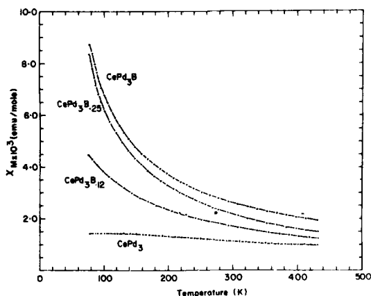
Figure 3. Temperature dependence of the susceptibility of \text{CePd}_3\text{B}_x ( x = 0, 0.12, 0.25 and 1.0 ) alloys.
