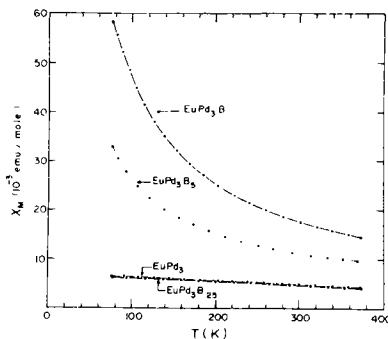
Figure 7. The temperature dependence of susceptibility of \text{EuPd}_3\text{B}_x ( x = 0, 0.25, 0.5 and 1.0 ) alloys.
