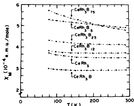
Figure 16. The temperature dependence of susceptibility of \text{CeRh}_3\text{B}_x ( x = 0, 0.12, 0.25, 0.5, 0.75 and 1.0 ) alloys.
