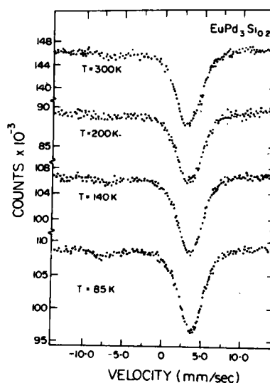
Figure 14. The temperature dependence of ^{151}\text{Eu} Mössbauer spectrum in \text{EuPd}_3\text{Si}_{0.25} .
