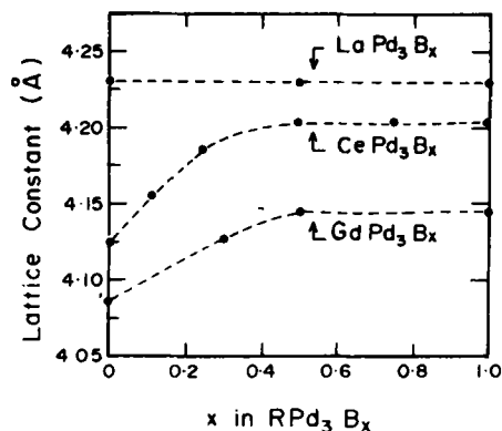
Figure 2b. Variation of lattice parameter as a function of boron concentration x in RPd_3B_x ( R = La, Ce and Gd) alloys.
