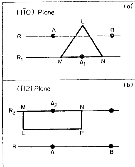
Figure 2. Regions where the potentials of the atoms of nearer \langle 110 \rangle rows of R dominate in the channels of two rows (one R , other R_1, R_2 ). (a) Region of the dominating field (the triangle LMN ) of an atom A_1 of the nearest \langle 110 \rangle row R_1 shown in the (110) plane. (b) Region of the dominating field (the rectangle LMNP ) of an atom A_2 of the \langle 110 \rangle row R_2 shown in the (112) plane.
