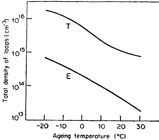
Figure 2. Temperature dependence of the total density of clusters.
