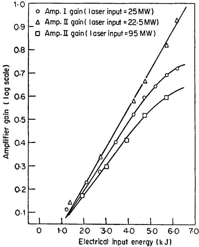
Figure 4. Gain characteristics of amplifiers
