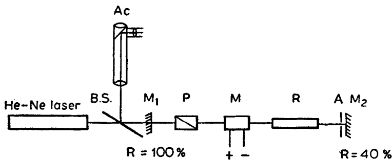
Figure 2. Schematic diagram of the oscillator
