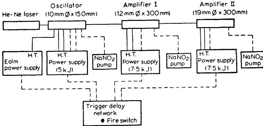
Figure 1. Block diagram of the laser system
