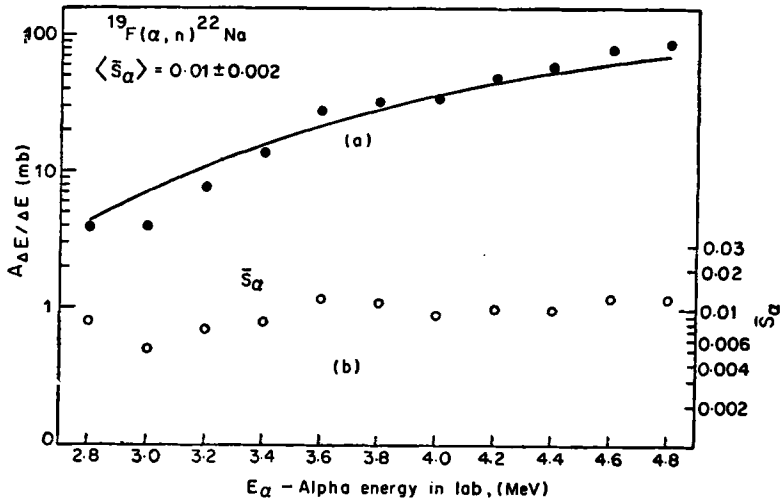
Figure 3. (a) Plot of A_{\Delta E}/\Delta E against the bombarding energy in MeV. (b) Plot of strength function \bar{S}_{\alpha} as a function of E_{\alpha} .
