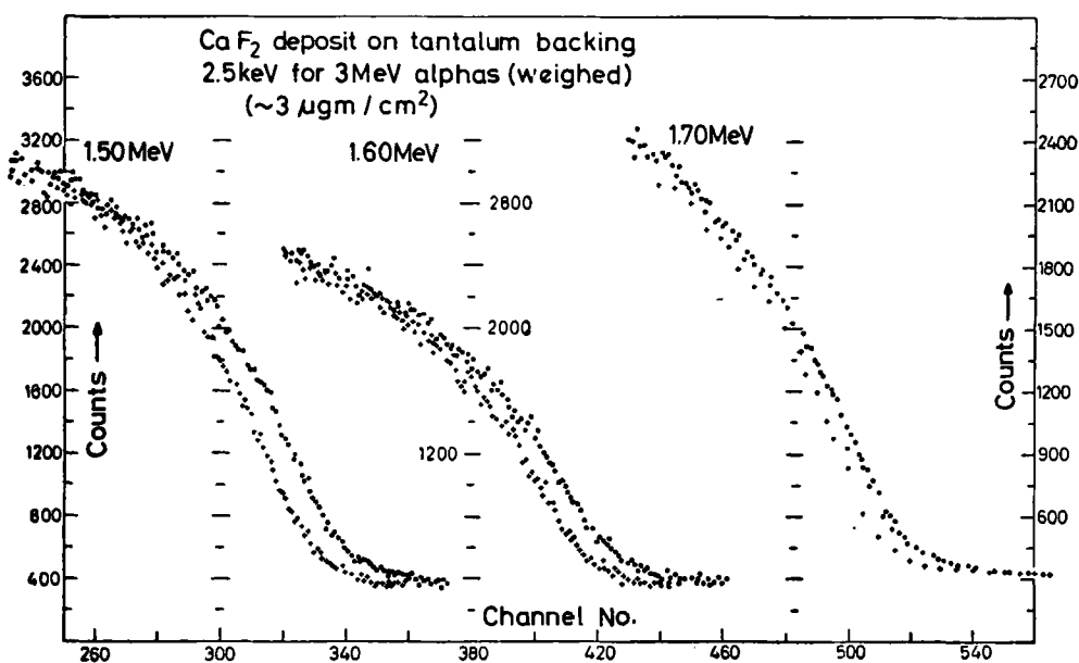
Figure 1. Typical alpha back scattered spectra indicating the decrease in energy loss as the incident alpha energy increases.
