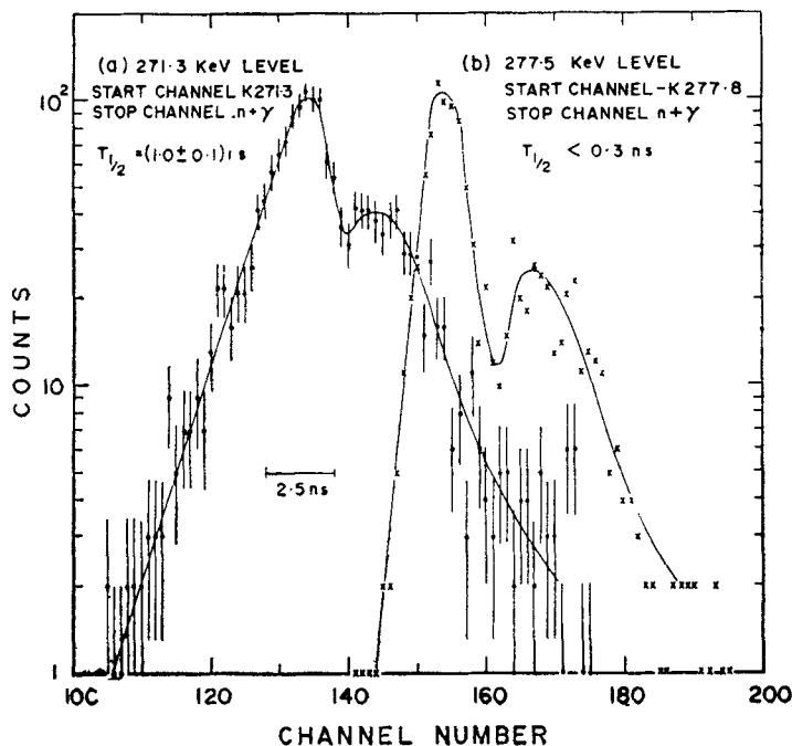
Figure 7. Decay curves for the 271.4 and 277.5 keV levels. K-conversion electrons corresponding to the 271.3 and 277.8 keV transitions were chosen in the start channel of TAC, and neutrons and \gamma -rays in the stop channel. Neutrons of energy greater than 50 keV were accepted in the fast channel.
