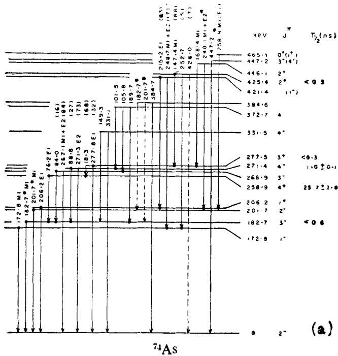
Figure 4. Proposed level scheme of ^{74}\text{As} . The branching ratios are indicated on top of the transitions. The decay properties of the low lying levels are shown in figure 4 a while those of the higher energy levels are shown in figure 4 b. The transitions indicated by an asterisk have been assigned at two places. The value of the half-life for the 258.9 keV level quoted in figure 4 a is obtained from the present work.
