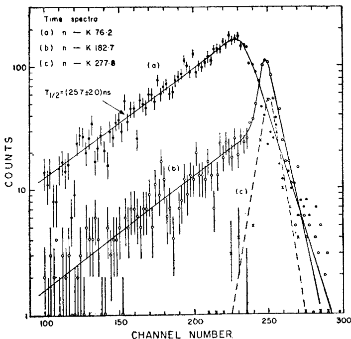
Figure 5. Time spectra obtained by choosing neutrons in the stop channel of TAC and the K-conversion lines corresponding to (a) 76.2, (b) 182.7 and (c) 277.8 keV transitions in the start channel.
