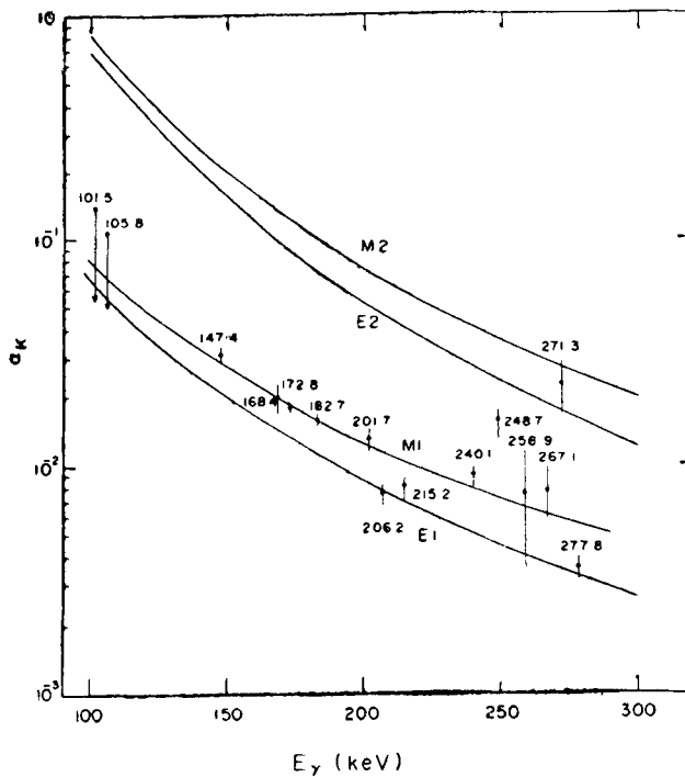
Figure 3. Comparison of the measured values of \alpha_k with theoretical values. The continuous lines are the values of \alpha_k taken from Hager and Seltzer (1968) for various multiplicities.
