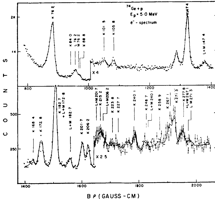
Figure 2. Internal conversion electron spectrum recorded with the six-gap spectrometer at E_p = 5.0 MeV. The numbers indicate the energies of the transitions in keV.
