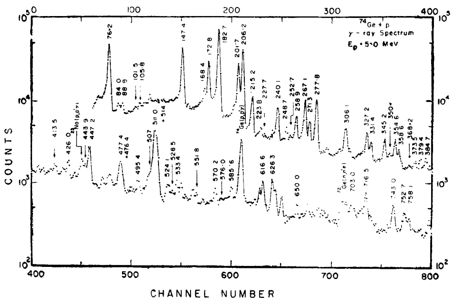
Figure 1. Gamma-ray spectrum obtained by proton bombardment of Germanium oxide enriched in ^{74}\text{Ge} ( \sim 95\% ) at E_p = 5.0 MeV using a 27\text{ cm}^3 Ge(Li) detector. The numbers indicate the gamma-ray energies in keV. The background gamma-rays are appropriately marked.
