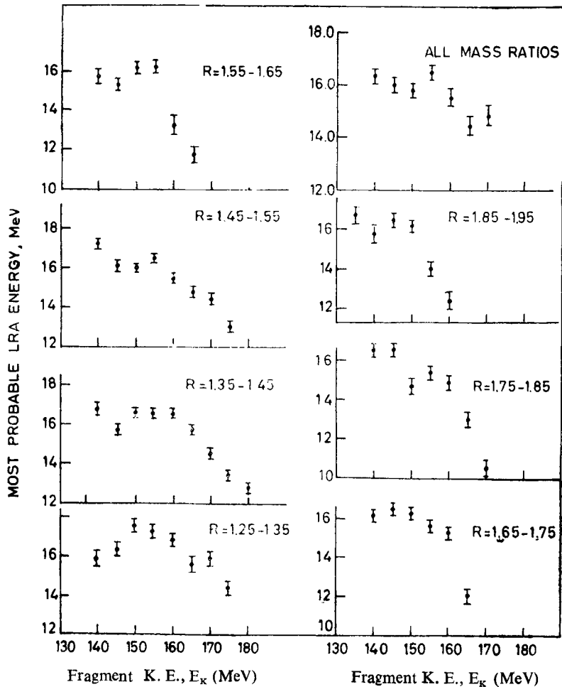
Figure 10. Most probable values of LRA energy as a function of fragment kinetic energy for various mass divisions.
