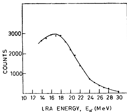
Figure 3. Summed up LRA spectrum of both the detectors.
