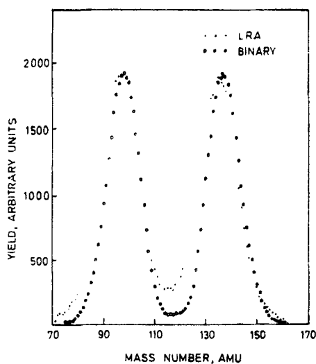
Figure 6. Mass distributions in binary and LRA fission.
