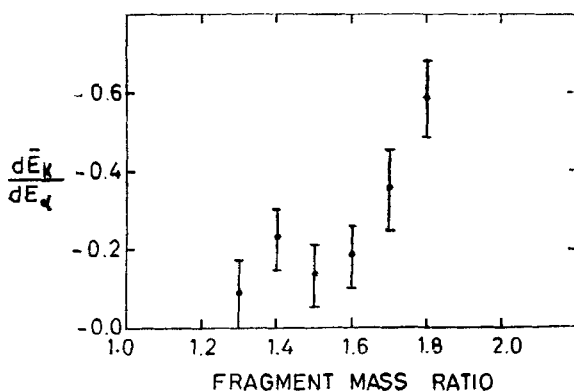
Figure 11. Variation of d\bar{E}_k/dE_\alpha with fragment mass ratio.
