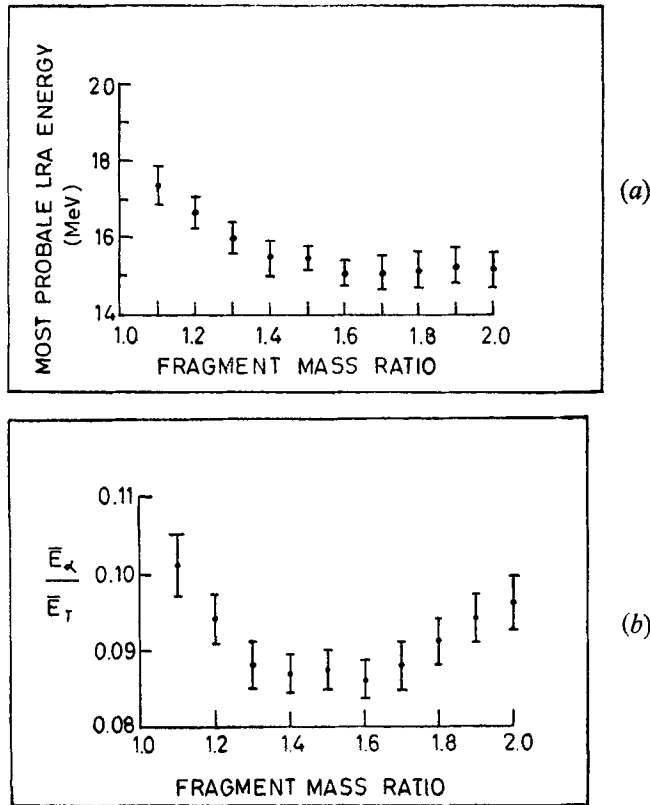
Figure 8. (a) Most probable values of LRA energy as a function of fragment mass ratio. (b) A plot of the quantity \bar{E}_\alpha/\bar{E}_T as a function of fragment mass ratio. \bar{E}_\alpha and \bar{E}_T are the most probable values of the LRA and total kinetic energy.
