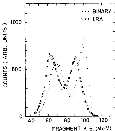
Figure 4. Kinetic energy distributions in binary and LRA fission.
