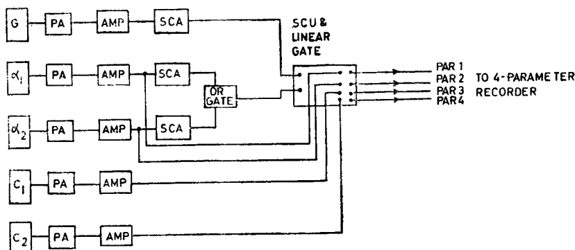
Figure 2. Block diagram of the electronic set up. PA—Pre-amplifier, AMP—Amplifier, SCA—Single Channel analyser, SCU—Slow Coincidence Unit.
