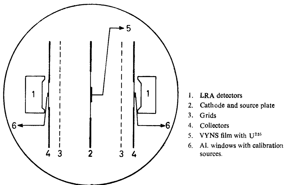
Figure 1. Schematic diagram of experimental assembly.
