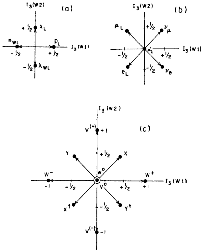
Figure 1. Weight diagrams of O_5 for (a) the left-handed (weak) quarks ( \sim \underline{4} ); (b) the left-handed leptons ( \sim \underline{5} ); and (c) the IVB's ( \sim \underline{10} ). Weight vectors are denoted by solid lines with arrows.
