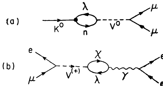
Figure 2. (a) Mechanism for the K^0 \rightarrow \mu\bar{\mu} decay via the V^0 . (b) Mechanism for the decay \mu \rightarrow ee\bar{e} via the V^{(+)} and the anomalous electromagnetic interaction.
