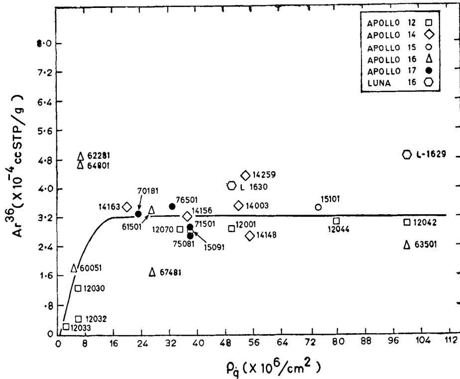
Figure 3. Correlation between the measured ^{36}\text{Ar} contents with the \rho_q (the quartile, track density) values given for several Apollo and Luna samples (Arrhenius et al 1971 and Bhandari et al 1972 and 1973). ^{36}\text{Ar} contents are taken from Hintenberger et al (1971), Heymann et al (1972), Pepin et al (1972), Kirsten et al (1972), Bogard et al (1972), Berdot et al (1972).
