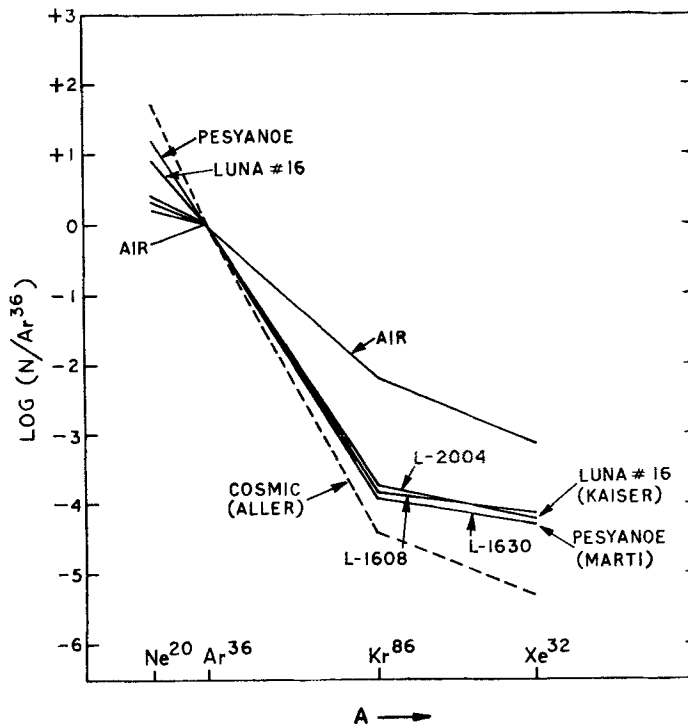
Figure 2. Abundance of trapped noble gases relative to ^{36}\text{Ar} observed in Luna 16 and 20 bulk soil samples. These data are compared with those of Pesyanoë (Marti 1969), and Luna 16 (Kaiser 1972) as well as cosmic abundances (Aller 1961) and air (Nier 1950). The lines representing Kaiser (1972) and Marti (1969) data could not be shown separately as they agree closely to those of L-1608, 1630 and 2004 for Ar, Kr and Xe. The deviations could be indicated only for Ne.
