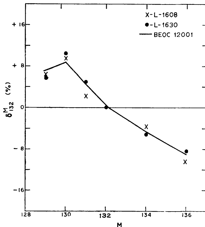
Figure 1. Comparison of the deduced isotopic Xe composition from Luna 16 soil fractions after correcting for spallogenic contribution, with the surface correlated solar Xe from BEOC-12001 data of Eberhardt et al (1972).
