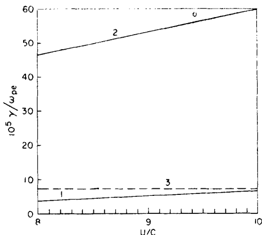
Figure 3. Variation of growth rate \gamma/\omega_{pe} versus U/c for a_{\parallel 0}/a_{\parallel i} = 100 , \omega_{pe}/ka_{\parallel e} = 10 , and a_{\parallel 0}/c = 0.1 and for n_b/n_p = 0.01 and 0.05 respectively. The broken curve 3, which is for the case when return currents are neglected but the other parameters are same as above, denotes damping. The damping remains unaffected by the increase of n_b/n_p . The value of the real frequency is \omega/\omega_{pe} = -5.17 \times 10^{-3} for all the curves.
