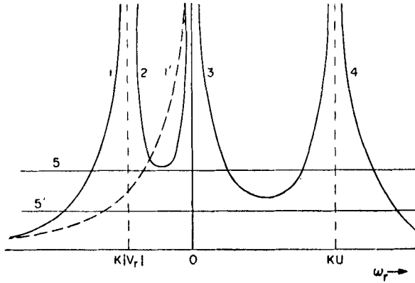
Figure 1. Schematic plot of eq. (10). Curves 1–4 are for F(\omega, k) and curves 5 and 5' are for F(\omega, k) = 1 . In the absence of return currents the curves 1 and 2 merge together and form the curve 1'. Curves 5 and 2 show instability.
