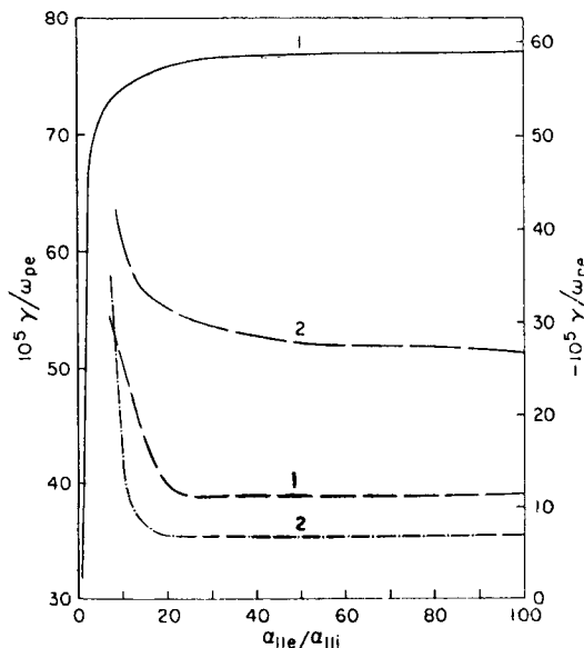
Figure 2. Variation of growth rate \gamma/\omega_{pe} (—) and real frequency \omega_r/\omega_{pe} (---) in the presence (curve 1) and absence (curve 2) of return currents versus \alpha_{||e}/\alpha_{||i} for n_b/n_p = 0.05 , U/c = 0.95 , \omega_{pe}/k\alpha_{||e} = 10 , and for \alpha_{||e}/c = 10^{-2} . The broken curve 2 (- · - · -) denotes damping and follows the scale given on the right hand side of the figure.
