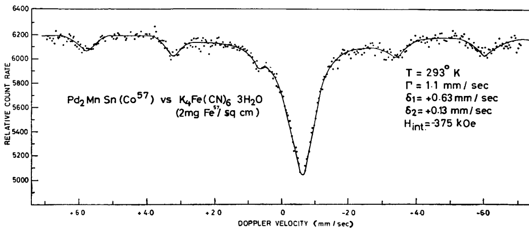
Figure 2. Mössbauer spectrum of Pd 2 MnSn(Co 57 ) at 293 K. Enriched K 4 Fe(CN) 6 ·3H 2 O containing 2 mg Fe 57 /cm 2 was used as an absorber.
