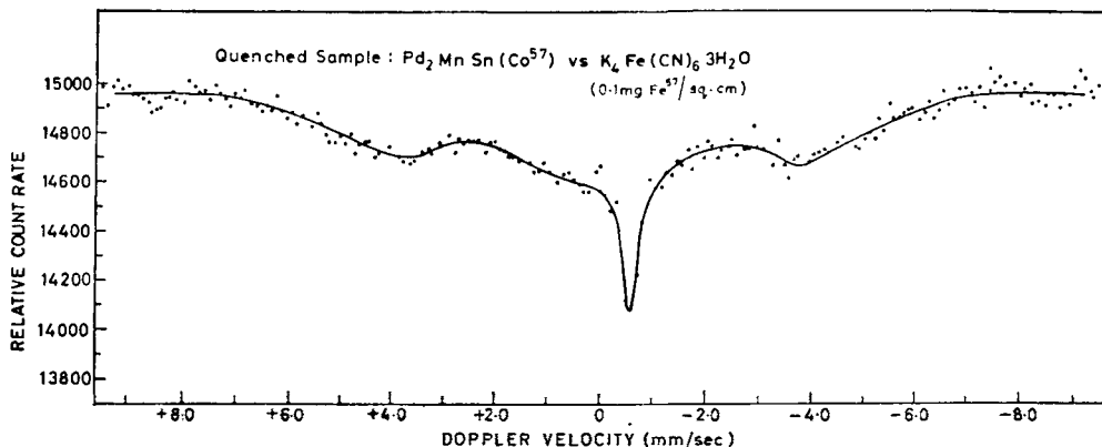
Figure 4. Mössbauer spectrum of \text{Pd}_2\text{MnSn}(\text{Co}^{57}) at 293 K. The source was quenched from 900°C. \text{K}_4\text{Fe}(\text{CN})_6\cdot 3\text{H}_2\text{O} containing 0.1 mg \text{Fe}^{57}/\text{cm}^2 was used as an absorber.
