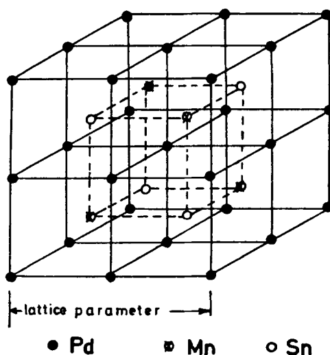
Figure 1. Heusler alloy structure
