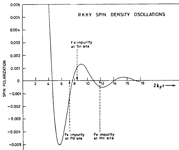
Figure 5. Unnormalized conduction electron spin polarization in \text{Pd}_2\text{MnSn} due to the localised magnetic moment on a Mn atom at the origin versus 2k_F r . Positions of \text{Fe}^{57} impurities occupying Pd- Sn and Mn sites are also shown.
