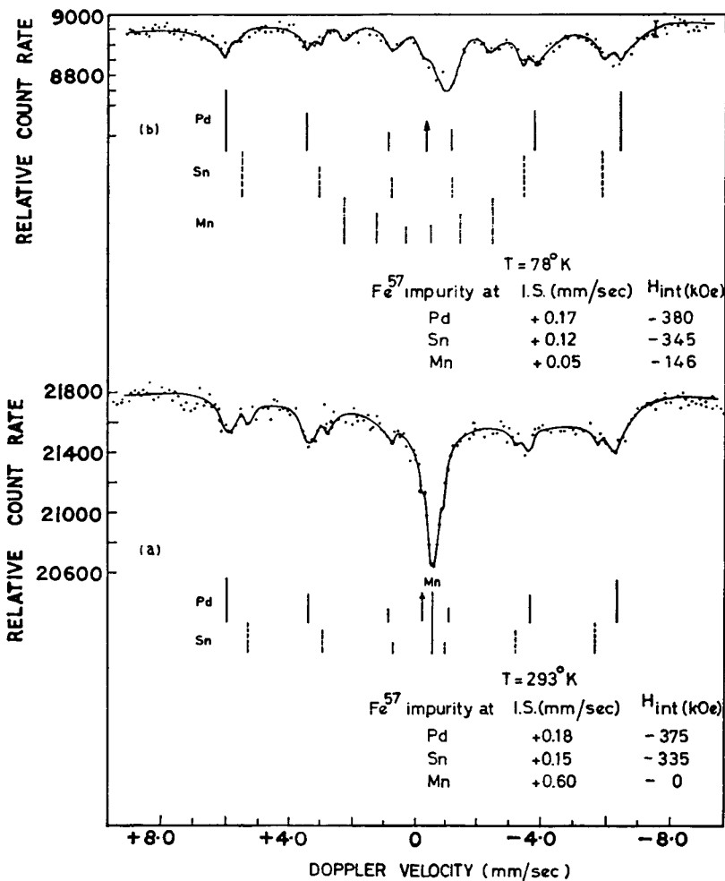
Figure 3. Mössbauer spectra of Fe 57 impurities in Pd 2 MnSn (a) at 293 K and (b) at 78 K. The absorber used was K 4 Fe(CN) 6 ·3H 2 O containing 0.1 mg Fe 57 /cm 2 .
