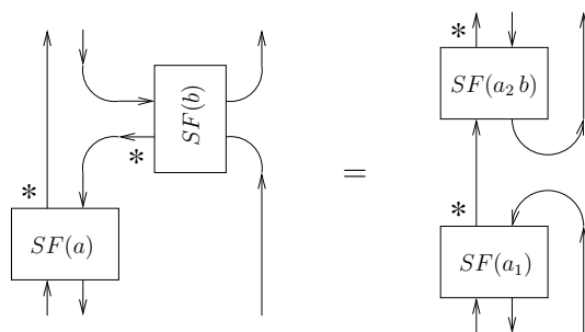
Figure 18. Relation to be verified in -P(H^*, \delta) .
