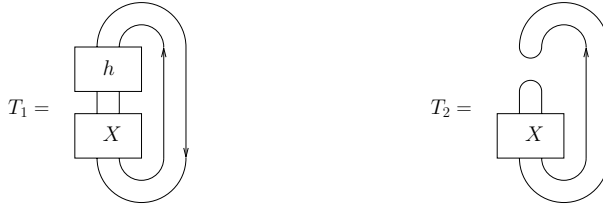
Figure 6. Two tangles that differ by the relation (I).
