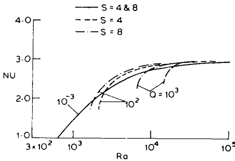
Figure 6. Curves of heat transport Nusselt number (Nu) against Rayleigh number (Ra) for viscous case P_r = 10^3 .
