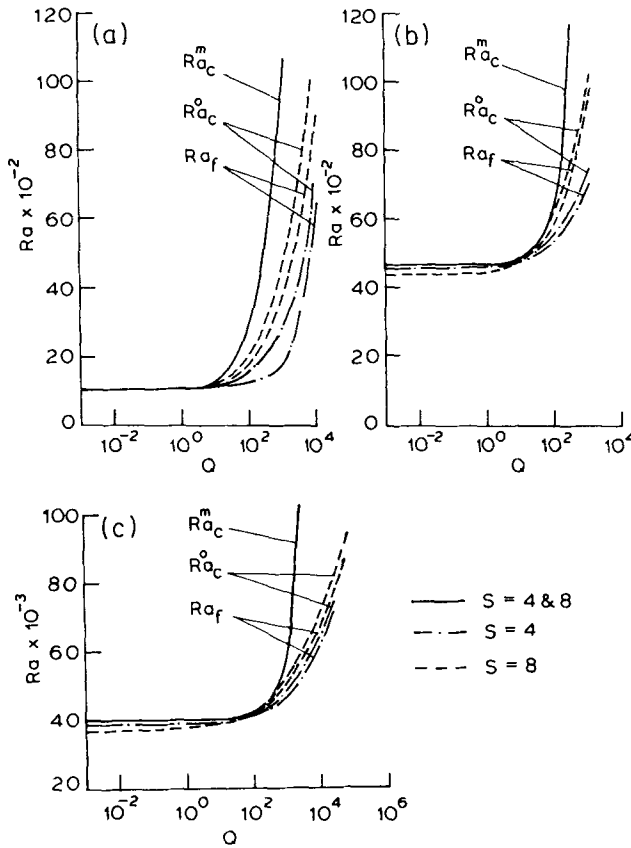
Figure 3. Curves of Ra^m , Ra^0 and Ra_f as function of Q for P_i = 10^{-1} , 10^{-2} and 10^{-3} (Brinkman model).
