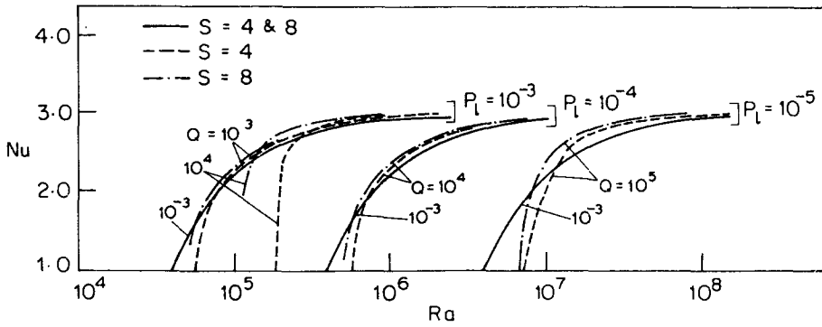
Figure 4. Curves of heat transport Nusselt number (Nu) against Rayleigh number (Ra) for (i) P_r = 10^{-3} (ii) P_r = 10^{-4} and (iii) P_r = 10^{-5} .
