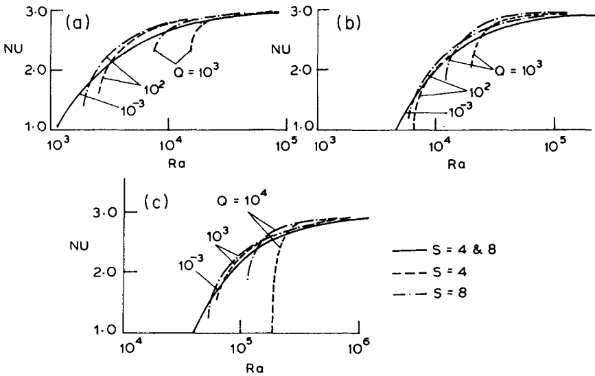
Figure 5. Curves of heat transport Nusselt number (Nu) against Rayleigh number (Ra) for Brinkman model (a) P_r = 10^{-1} (b) P_r = 10^{-2} and (c) P_r = 10^{-3} .
