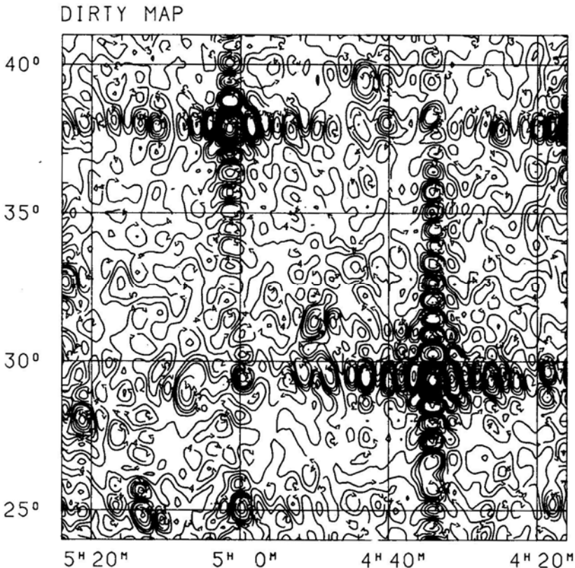
Figure 5. Dirty map of 1 \text{ hr} \times 15^\circ in extent observed in the present survey. The two strong sources 3C 123 ( \alpha = 04^{\text{h}}34^{\text{m}} ; \delta = 29^\circ 23' ) and 3C 134 ( \alpha = 05^{\text{h}}01^{\text{m}} ; \delta = 37^\circ 51' ) and their sidelobes are clearly seen.
