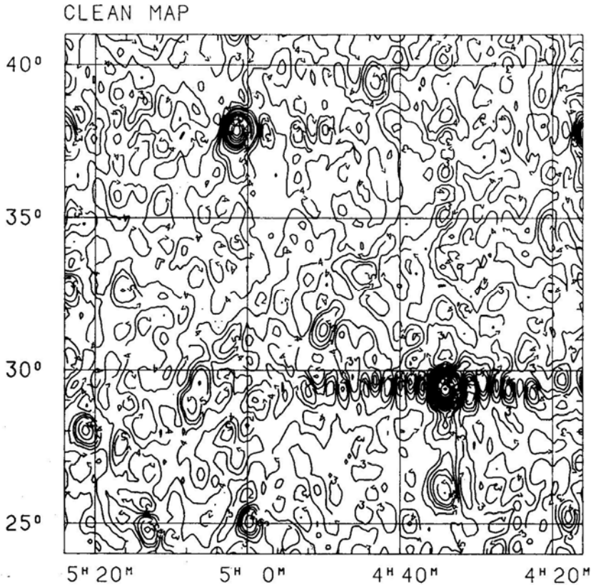
Figure 6. CLEANed map of the region shown in Fig. 5 obtained through the algorithm indicated in Fig. 4. Note that a weak source ( \alpha=04^{\text{h}} 34^{\text{m}} ; \delta = 26^{\circ}04' ) which was buried in the sidelobes of 3C 123 (Fig. 5) is clearly seen here.
