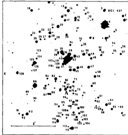
Figure 1. Finding chart for the field of Czernik 20 (OC1427), reproduced from the Palomar Observatory Sky Survey (POSS) charts. The identification numbers are introduced in the present work.
