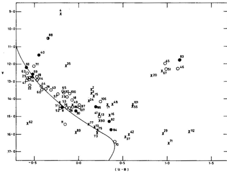
Figure 5. The (U - B) versus V magnitude diagram of the stars in the field of OC1 427. The solid curve represents the ZAMS ( cf. Schmidt-Kaler 1982) which is shifted to match with the observations. The symbols are same as in Figs 3 and 4.
