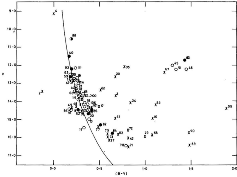
Figure 4. The (B - V) versus V magnitude diagram of the stars in the field of OC1 427. The solid curve represents the zero-age main sequence (ZAMS) ( cf. Schmidt-Kaler 1982), which is shifted to match with the observations. The symbols are same as in Fig. 3.
