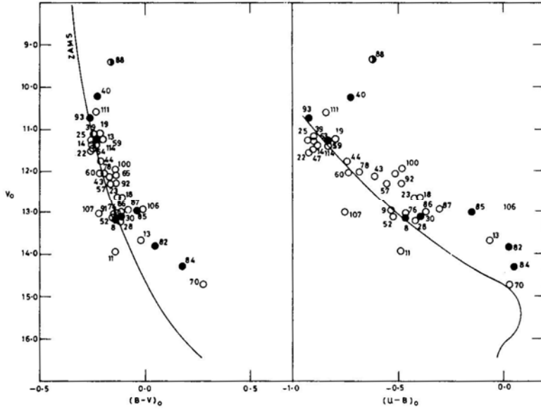
Figure 6. The intrinsic (B - V)_0 , V_0 and (U - B)_0 , V_0 diagrams of OC1 427. The solid curves represent the respective ZAMS taken from Schmidt-Kaler (1982). The symbols are same as in Figs 3–5, with all the non-members- deleted.
