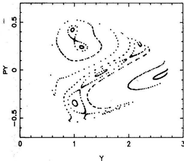
Figure 3. Surface of section ( x=1 , p_x>0 ) for \mathcal{H} = -0.45 .
