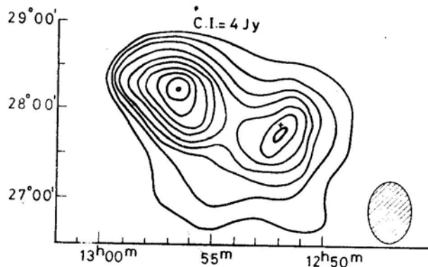
Figure 1. Map of the Coma cluster region at 34.5 MHz obtained with the low-frequency radio telescope at Gauribidanur. The contour interval is 4 Jy/beam. The lowest contour corresponds to 4 Jy/beam and is significant at the 3-sigma level. The position of the radio galaxy Coma A is shown by a cross.
