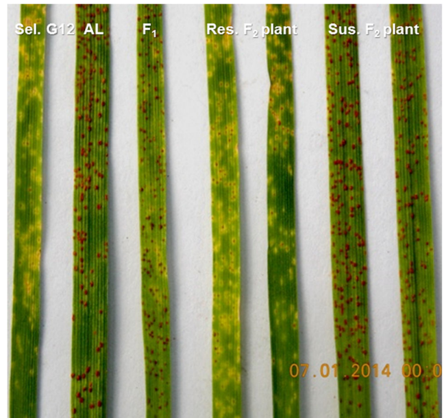
Figure 1. Infection types (ITs) of pathotype 77-5 on Selection G12, Agra Local, F 1 and for F 2 plants of the cross, Selection G12/AL.
