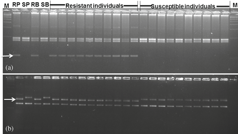
Figure 2. Bulked segregant analysis and co-segregation of SSR marker (a) Xgwm547 and (b) Xgwm114 with the leaf rust resistant gene; M, 100 bp ladder; RP, resistant parent (Selection G12); SP, susceptible parent (Agra Local); RB, resistant bulk; SB, susceptible bulk; bulked sample is based on homozygous F_2 plants.
