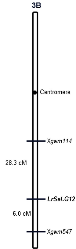
Figure 3. Position of LrG12 on the genetic map of wheat chromosome 3BL.
