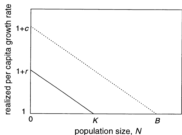
Figure 2. The linear density dependence of realized per capita population growth rate assumed in the model of Hallam and Clark (1981). Here the coefficient of competition a = c/B , and this slope determines the equilibrium population size K .
