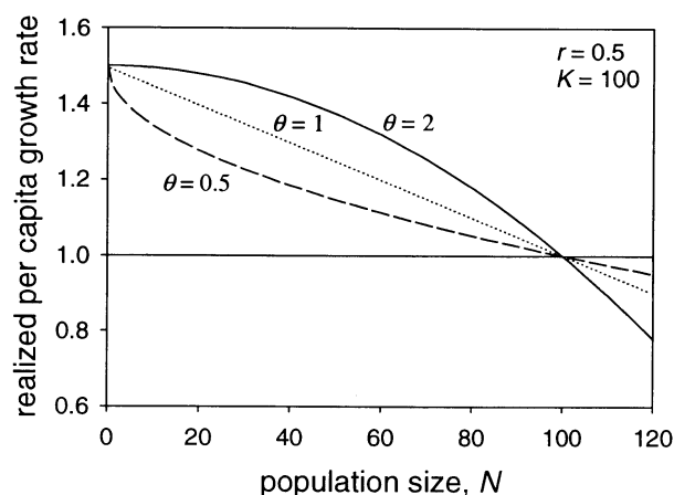
Figure 3. The density dependence of realized per capita population growth rate according to the formulation of Gilpin et al. (1976) shown here for some arbitrary values of r , K and q . Here the density dependence can be nonlinear, depending on the value of the parameter q ( q = 1 reduces to the logistic case). Note that if there were three genotypes with identical r and K values as depicted here, the one with q = 2 would be able to sustain higher realized growth rates than the others at all population densities from 0 to K .
