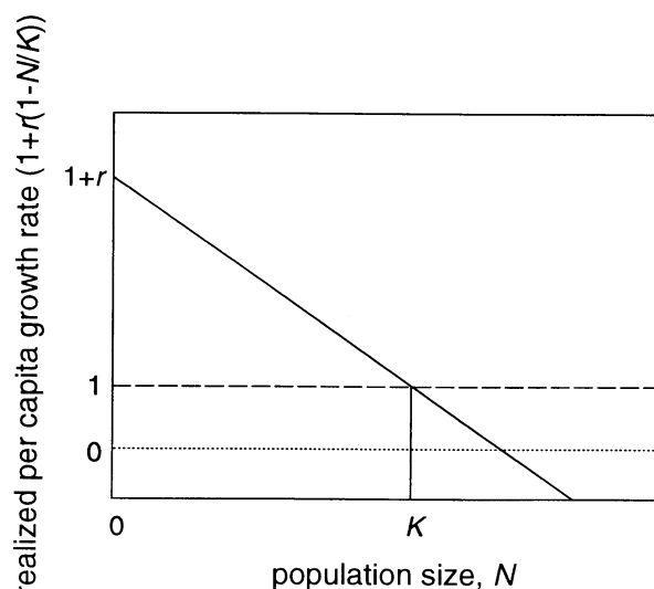
Figure 1. The linear density dependence of realized per capita population growth rate assumed in the logistic model. When N = K , the realized per capita growth rate is 1 and thus K is the equilibrium population size, as well as the saturation capacity of the environment. The slope of the line ( r/K ) is the coefficient of competition a in this formulation.
