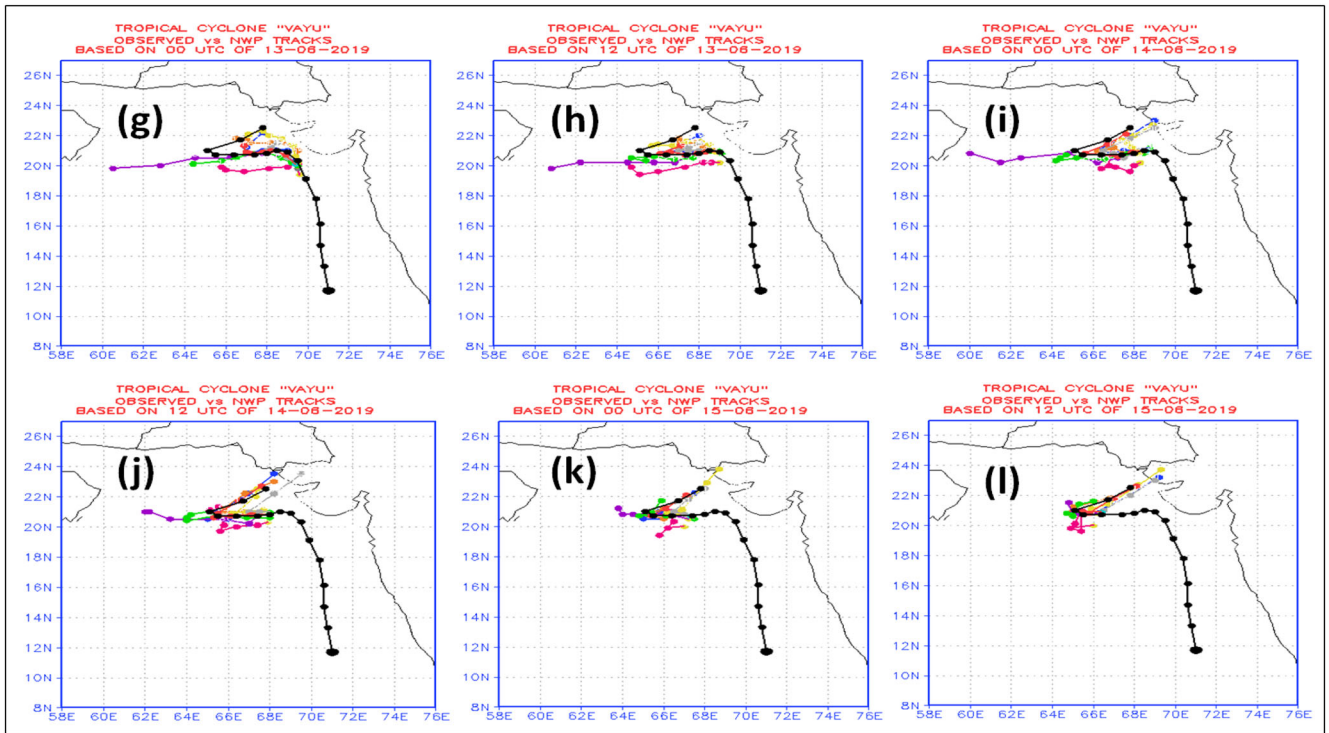
Figure 3. (a-l) Forecast tracks by different models based on 00 and 12 UTC during 10–15th June along with observed tracks.
