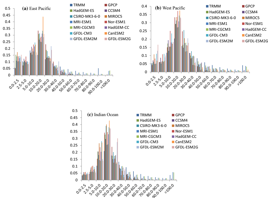
Figure 2. Rainfall PDF over East, and West Pacific, Indian Ocean from TRMM, GPCP, and CMIP5 models. The ranges of rain rate are (mm day -1 ) along X axis and rainfall PDF (in fraction) along Y axis.
