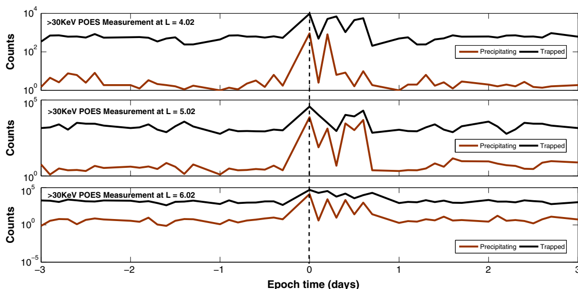
Figure 5. Superposed epoch plot of trapped and precipitating >30 keV electron from NOAA/POES satellite. The black line in each plot indicates measurements from 90° telescope (trapped electrons) while the red line indicates measurements from 0° telescope (precipitating electrons). The dash vertical line indicates arrival of SI (top is the >30 keV at L = 4.02 , middle is L = 5.02 while bottom is counts at L = 6.02 ).
