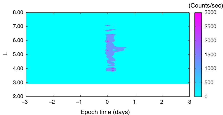
Figure 4. Superposed L-t deposition of >30 keV electron flux from MPED onboard POES satellites during SI-driven dropouts, based on MCETM calculations.
