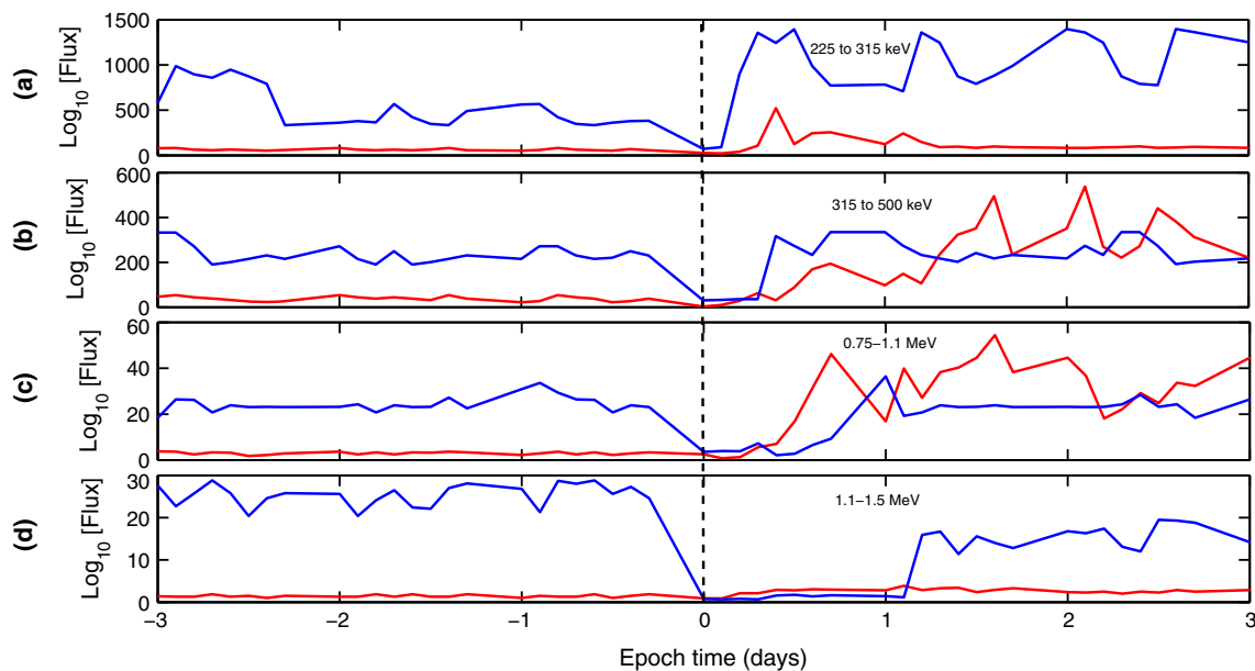
Figure 3. Superposed epoch plots of electron flux during SI-driven dropouts (blue line) and MC-driven dropouts (red line) as measured by combined LANL SOPA satellites: (a) 225–315 keV, (b) 315–500 keV, (c) 0.75–1.1 MeV, and (d) 1.1–1.5 MeV.
