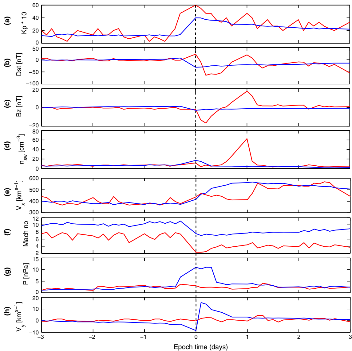
Figure 2. Plots of superposed properties of SI-driven dropouts (blue line) and MC-driven dropouts (red line) used. The zero epoch taken as SI onset are indicated by vertical line. From top is Kp, Dst, IMF Bz, solar wind number density, solar wind radial velocity, Alfvén Mach number, solar wind pressure and the solar wind azimuthal (west–east) flow velocity.
