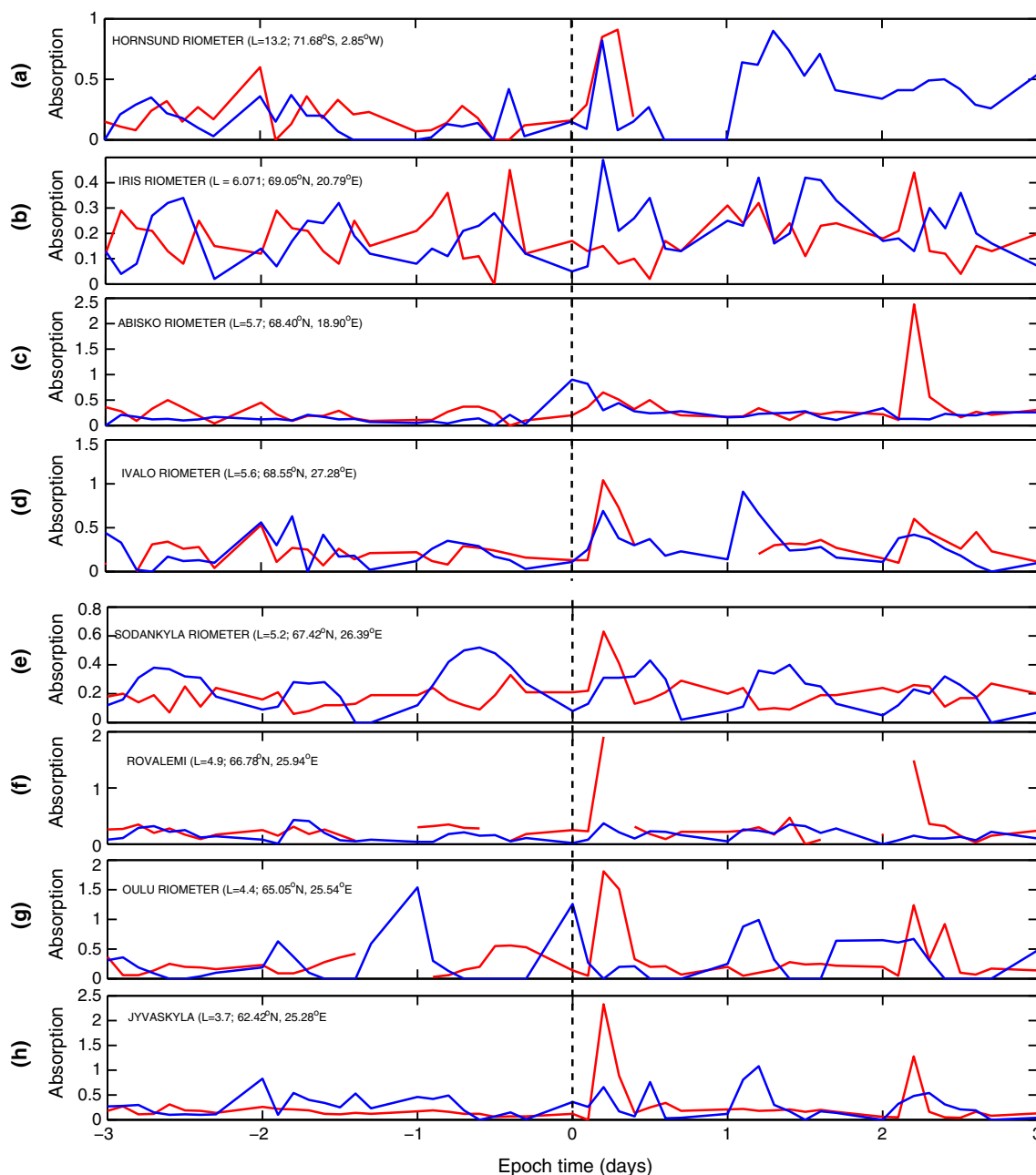
Figure 7. Superposed epoch of individual Finnish riometer absorption during SI-driven dropouts (blue line) and MC-driven dropouts (red line). From (a–h) is Hornsund, Iris, Abisko, Ivalo, Sodankylä, Rovaniemi, Oulu and Jyväskylä. The vertical line indicates onset of events.
