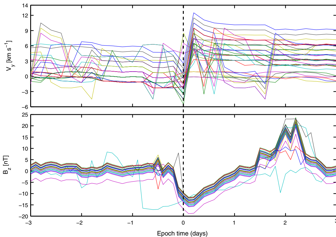
Figure 1. The solar wind azimuthal velocity (GSE- V_Y ) for set of the 80 SI (top panel) and IMF B_z for the set of MC (bottom).
