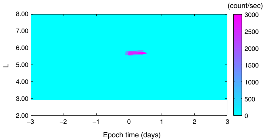
Figure 6. Superposed L–t deposition of >30 keV electron flux from MPED onboard POES satellites during MC-driven dropouts, based on MCETM calculations.
