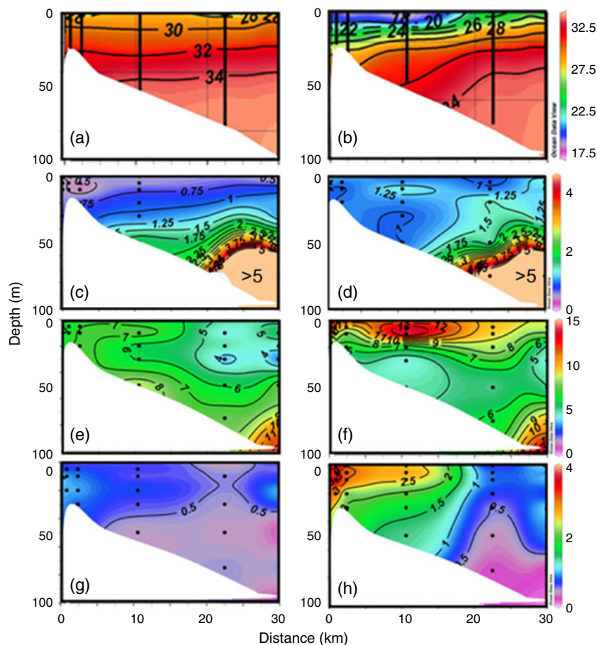
Figure 2. Variation of salinity (a, b), nitrate ( \mu\text{mol kg}^{-1} ; c, d), silicate ( \mu\text{mol kg}^{-1} ; e, f) and Chlorophyll a ( \text{mg m}^{-3} ; g, h) during October 2006 (normal) and October 2007 (after extreme rainfall event), respectively.
