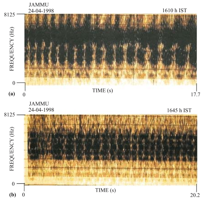
Figure 1. Typical examples of pulsing hiss recorded at Jammu during daytime (a) on 24 April 1998 at 16:10 h IST and (b) on 24 April 1998 at 16:45 h IST.
