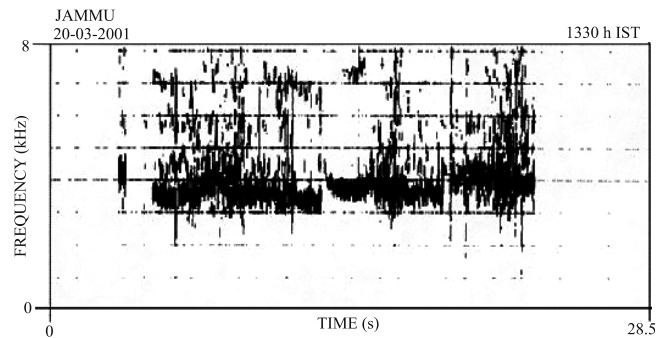
Figure 4. Typical example of pulsing VLF hiss emission of longer period recorded during daytime at Jammu on 20 March 2001 at 13:30 h IST.
