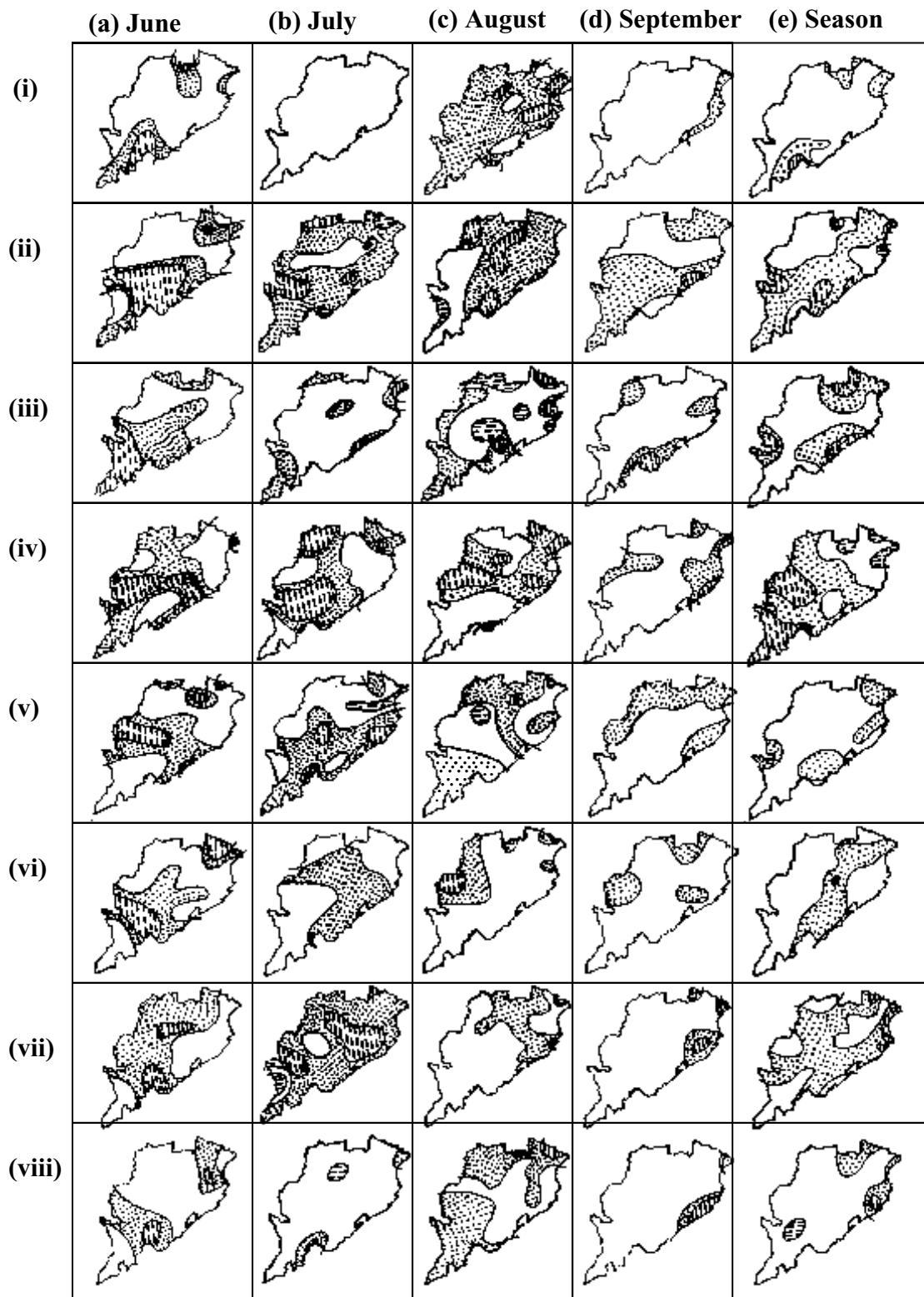
Regions of LPS: (i) NE Bay (ii) NW Bay (iii) WC Bay (iv) Orissa (v) East MP & Chhatishgarh (vi) Jharkhanda (vii) GWB (viii) Bangladesh ... Positive CC ||| Positive CC Significant at 90% confidence level □ Negative CC == Negative CC Significant at 90% confidence level
