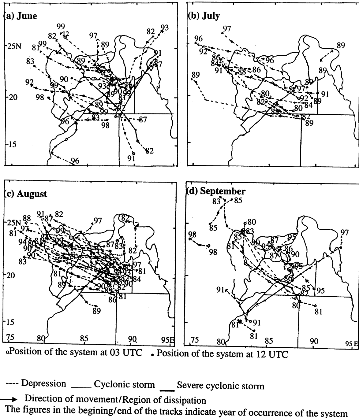
Figure 3. The tracks of cyclonic storms and depressions developing over Bay of Bengal during monsoon season (June–September) over a period of 20 years (1980–1999).
