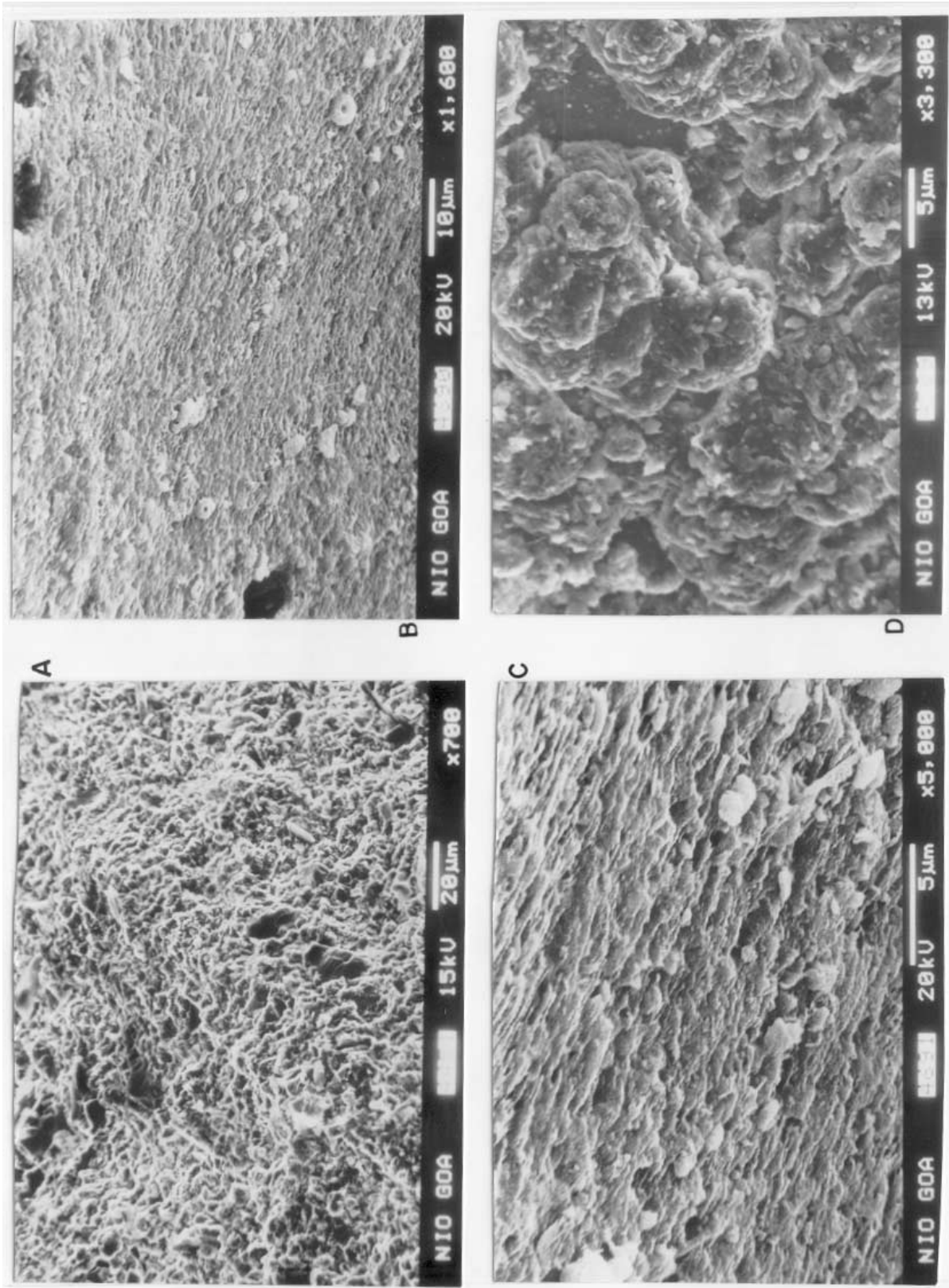
Figure 5. SEM photomicrographs of dolomite crusts from the carbonate platform. (A) Wrinkled dolomitized microlaminations of cyanobacteria, (B) cyanobacterial mats with trapped sediment detritus, (C) enlargement of 'B', and (D) ovoid to rounded dolomite microparticles and their aggregations, resembling bacterial aggregates.
