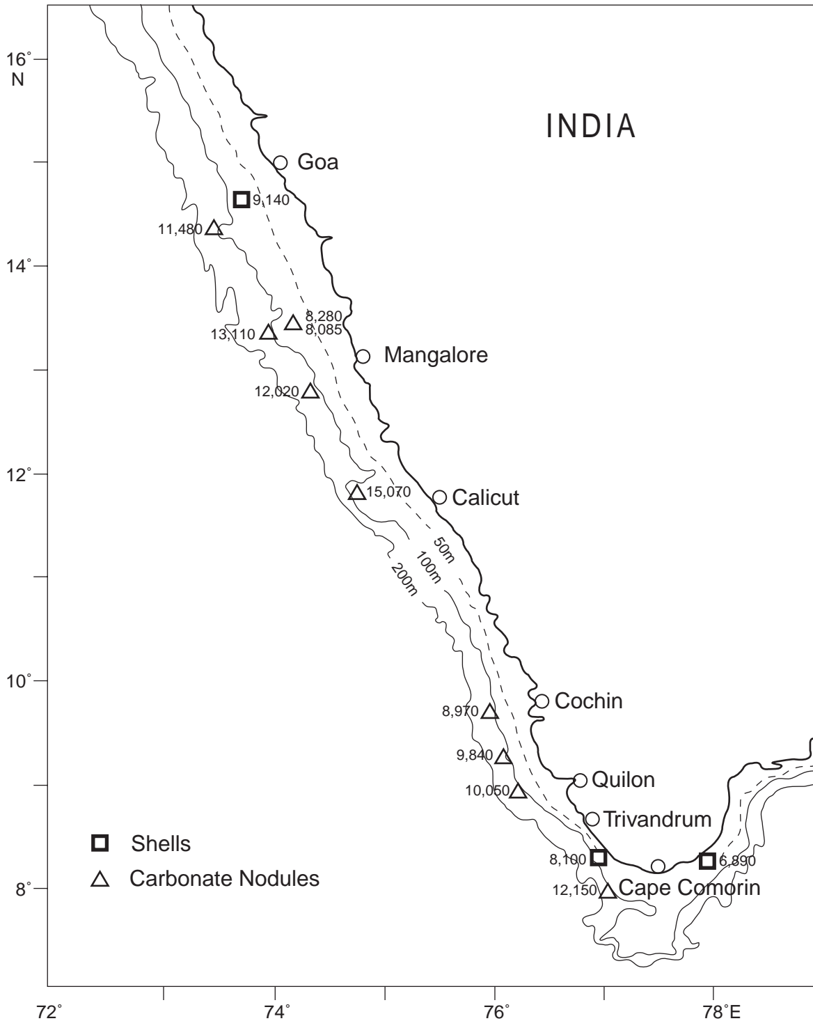
Figure 2(c). Measured radiocarbon ages of the samples off Goa-Cape Comorin.
