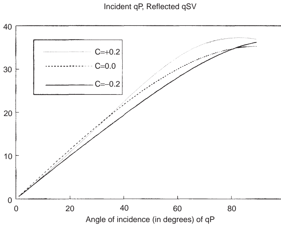
Figure 3. Variation of the angle of reflection ( e_4 ) of qSV waves with the angle of incidence ( e_1 ) of qP waves.
