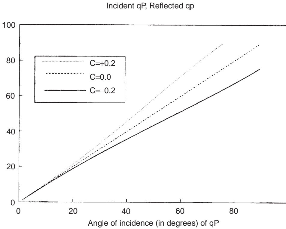
Figure 2. Variation of the angle of reflection ( e_3 ) of qP waves with the angle of incidence ( e_1 ) of qP waves for three values of the anisotropy parameter C .
