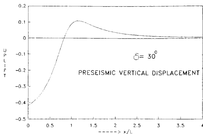
Figure 3. Profile of figure 2 reflected about the x -axis. Assuming complete elastic rebound during an earthquake, if figure 2 represents coseismic vertical displacement, then figure 3 represents preseismic vertical displacement.
