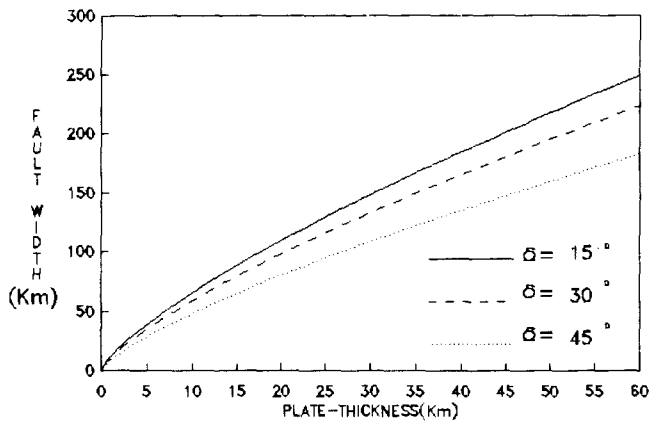
Figure 5. Fault-width for the two-dimensional dip-slip fault model for \delta = 15^\circ, 30^\circ, 45^\circ corresponding to the plate model of a given thickness with line shear force end loading.
