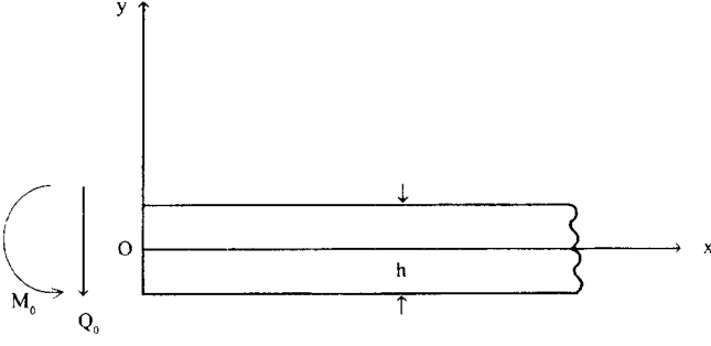
Figure 4. Geometry of a semi-infinite plate of thickness h under end loading, which is either a shear force Q_0 or a bending moment M_0 . The plate is terminated at the origin by the fault and extends to infinity in the positive x -direction.
