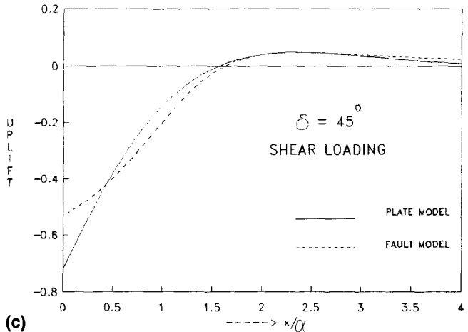
Figure 6(a, b and c). Variation of the vertical (up) displacement with distance for the dip-slip fault model and the plate model with shear loading for (a) \delta = 15^\circ ; (b) \delta = 30^\circ ; (c) \delta = 45^\circ . The displacement is measured in units of the slip b of the fault model.
