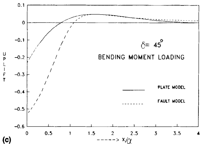
Figure 7(a, b and c). Variation of the vertical (up) displacement with distance for the dip-slip fault model and the plate model with bending moment loading for (a) \delta = 15^\circ ; (b) \delta = 30^\circ ; (c) \delta = 45^\circ . The displacement is measured in units of the slip b of the fault model.
