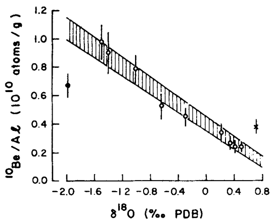
Figure 3. 10 Be/Al ratio versus \delta^{18}\text{O} plot for EN32 PC6. The shaded band represents the best-fit-line with errors. Sample E5, shown as a black dot ( \delta^{18}\text{O} = -1.98\text{‰} ), and E8 (denoted by X) are not used in the regression analysis. See text for discussion.
