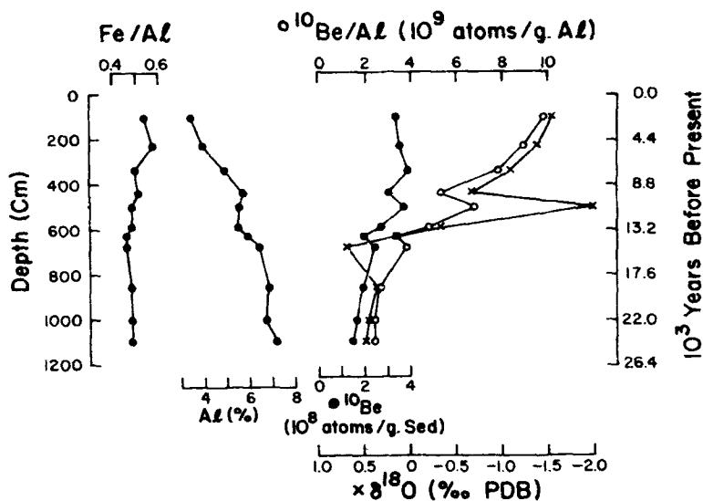
Figure 2. On the left are shown the Al and Fe/Al variations with depth. On the right side are shown the variations of ^{10}\text{Be} , ^{10}\text{Be}/\text{Al} and \delta^{18}\text{O} in the samples analysed. It is clear that ^{10}\text{Be}/\text{Al} variations show a more pronounced correlation with \delta^{18}\text{O} than with ^{10}\text{Be} (Somayajulu et al 1991). Notice that the \delta^{18}\text{O} scale is reversed to show the effect similar to the ^{10}\text{Be}/\text{Al} increase.
