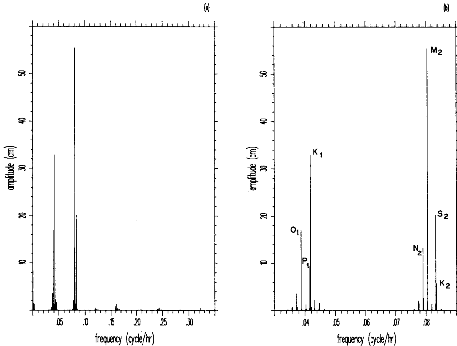
Figure 4. (a) Amplitude (cm) of the 69 most significant constituents at Marmagao. The horizontal axis gives frequency (cycle/hour). (b) Same as (a) but for only the diurnal and semi-diurnal constituents which dominate the tides at Marmagao. The enhanced resolution of the horizontal axis permits identification of the more prominent species.
