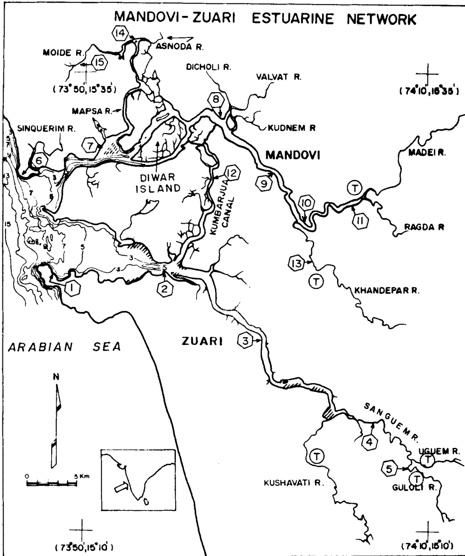
Figure 1. Map of the Mandovi-Zuari estuarine network based on publications from the Survey of India (1967), the Naval Hydrographic Office, India, and the Admiralty, U.K. The depth contours are with respect to mean sea level which is 1.3 m above Spring Low Water at Marmagao. To avoid clutter, the depth contours are shown only near the mouths of the main channels of the Mandovi and the Zuari. See figure 2 for variation of depth along the rest of the main channels. 'T' in a circle shows location up to which tidal influence is felt in the rivers Kushavati, Uguem, Guloli, Khandepar and Mandovi. The 15 locations where observations were made during April and August 1993 are shown with a number inside a hexagon. The correspondence between the numbers and the locations is as follows. 1: Marmagao; 2: Cortalim; 3: Loutulim; 4: Sanvordem; 5: Sanguem; 6: Aguada; 7: Penha de Franca; 8: Sarmanas; 9: Volvoi; 10: Sonarbaag; 11: Ganjem; 12: Banastarim; 13: Khandepar; 14: Sirsai; 15: Mappa.
