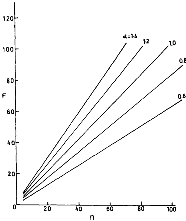
Figure 3. Variation of the roots of the frequency equation (22) with n for \alpha = 0.6, 0.8, 1.0, 1.2 and 1.4 .
