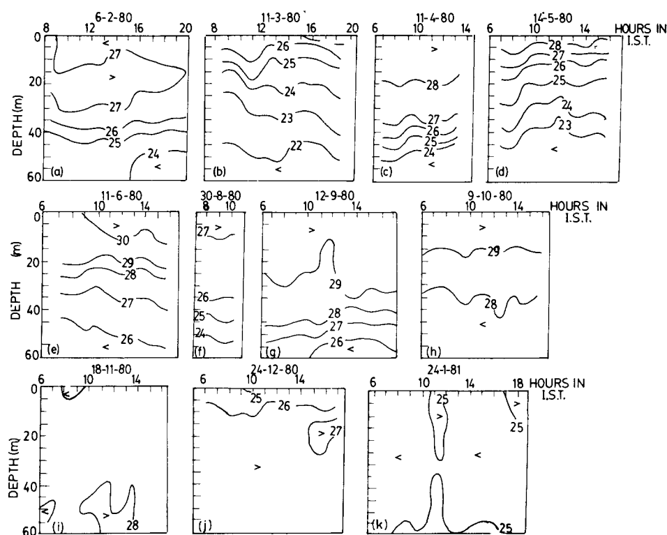
Figure 2. Diurnal variation of temperature(°C) in the coastal waters off Visakhapatnam for different months.
