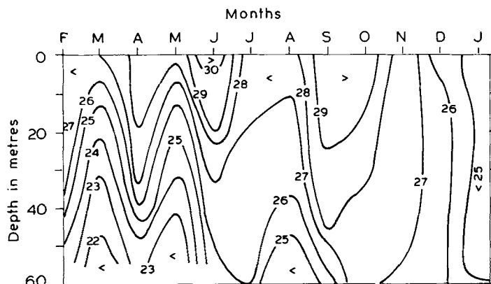
Figure 3. Seasonal variation of temperature(°C) in the coastal waters off Visakhapatnam.
