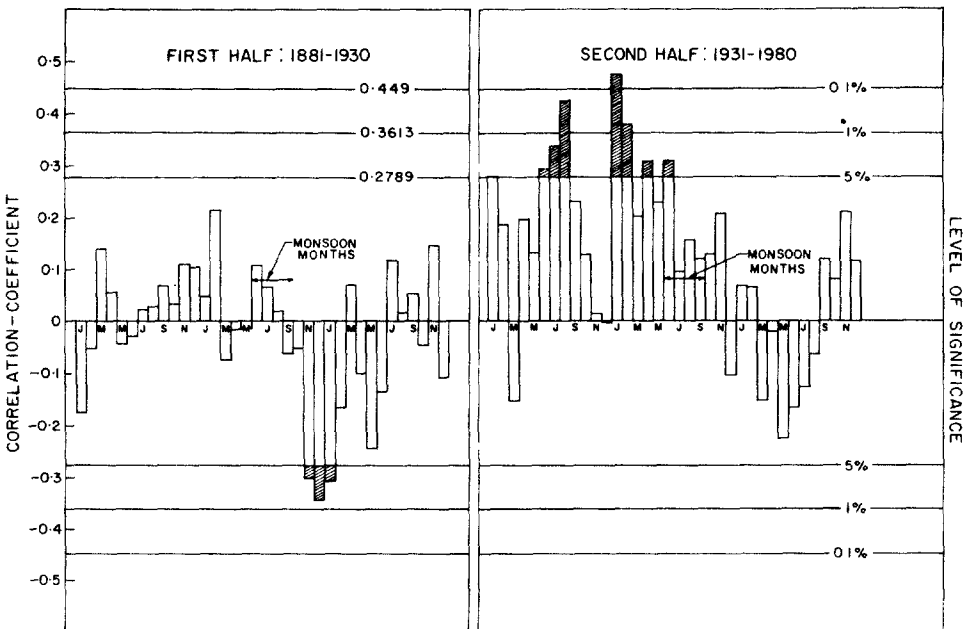
Figure 4. As in figure 3, except that the 100-year series is split into two equal series of 50 years.
