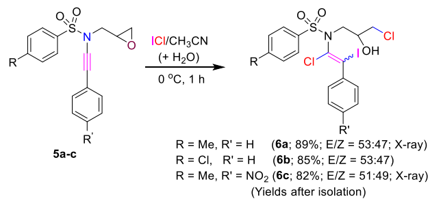
Scheme 6. Reaction of epoxy ynamides with ICl.
