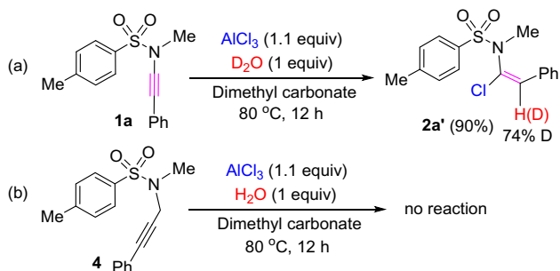
Scheme 5. Control Experiments.
