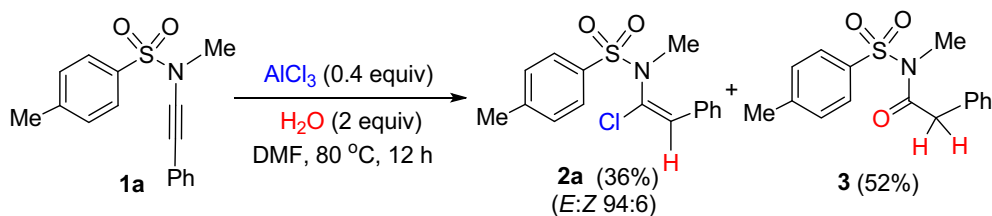
Scheme 3. Reaction of ynamide 1a with \text{AlCl}_3 affording products 2a and 3 .
