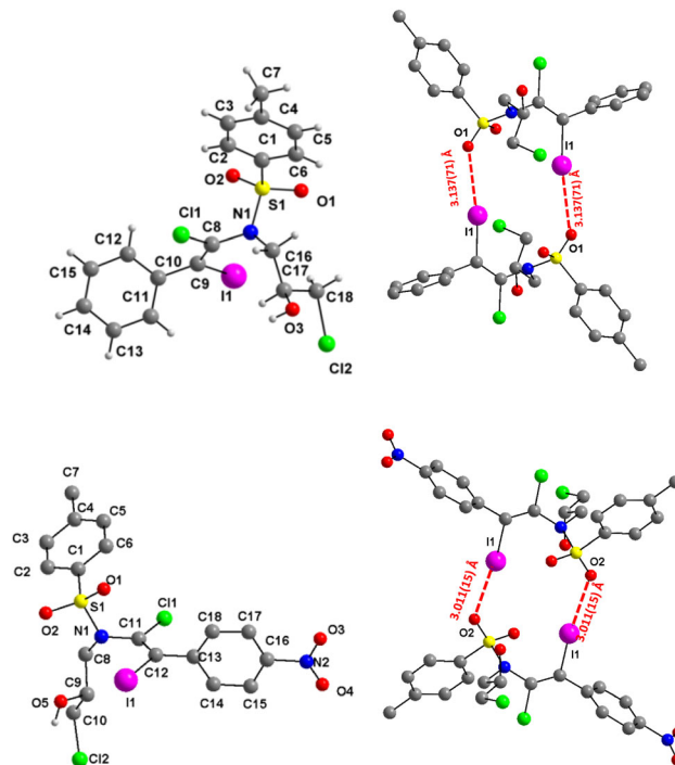
Figure 2. Molecular structures of compounds 6a (Top; CCDC 2033592) and 6c ·CH 2 Cl 2 (Bottom, solvent molecule is omitted; CCDC 2033593). Selected bond lengths [Å] with esds in parentheses: 6a I1-C9 2.099(7), C9-C8 1.340(10), C11-C8 1.754(8), C16-C17 1.494(15), C18-C17 1.44(2), O3-C17 1.550(18), C12-C18 1.908(15), I...O 3.137(71). 6c ·CH 2 Cl 2 I1-C12 2.116(10), C11-C12 1.315(13), C12-C13 1.447(13), C11-C11 1.747(10), C12-C10 1.789(15), O5-C9 1.464(16), N1-C11 1.411(12), I...O 3.011(15). Data quality for 6c was only moderate but structure could be readily refined. The I...O distances are considerably shorter than the sum of the corresponding van der Waals radii of O (1.52 Å) and I (1.98 Å) i.e. they are <3.50 Å [Note: Average I-O covalent bond distance: 2.14 Å].
